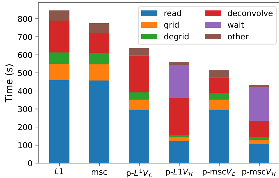
Sgr C
