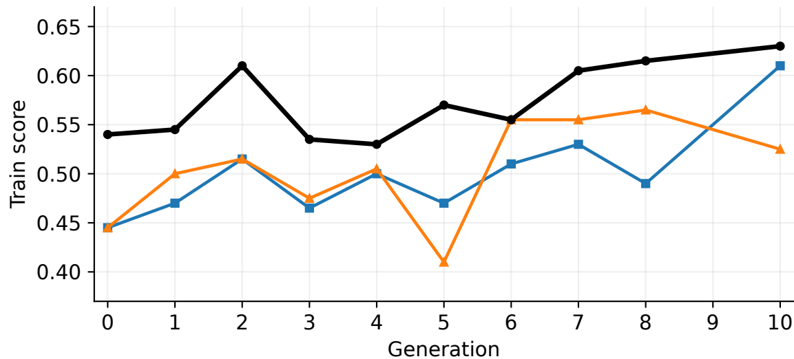
Train score
