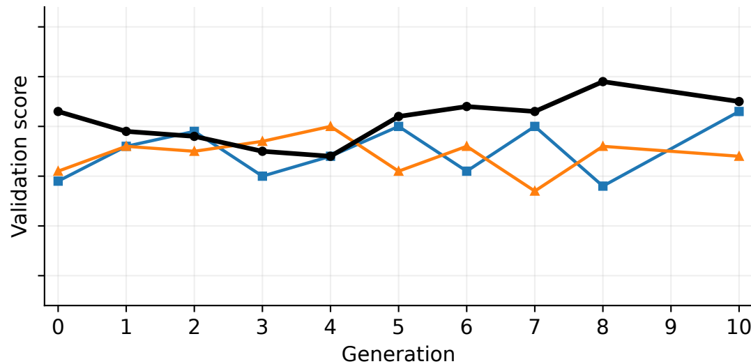
Validation score
