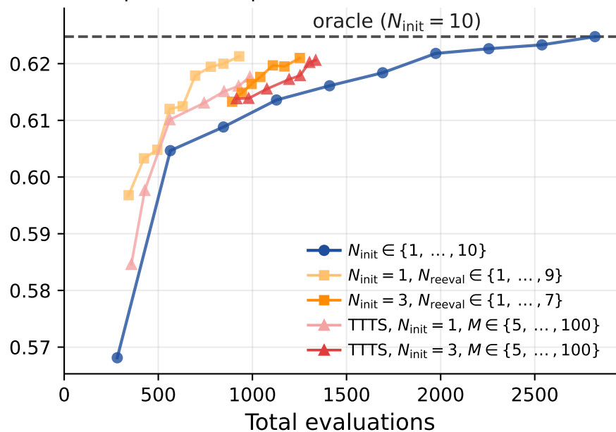
(c) Expected true parent fitness
