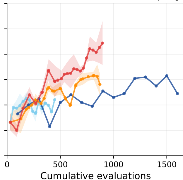
(b) Reevaluated fitness of best offspring
