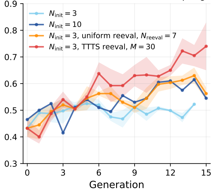
(a) Reevaluated fitness of best offspring
