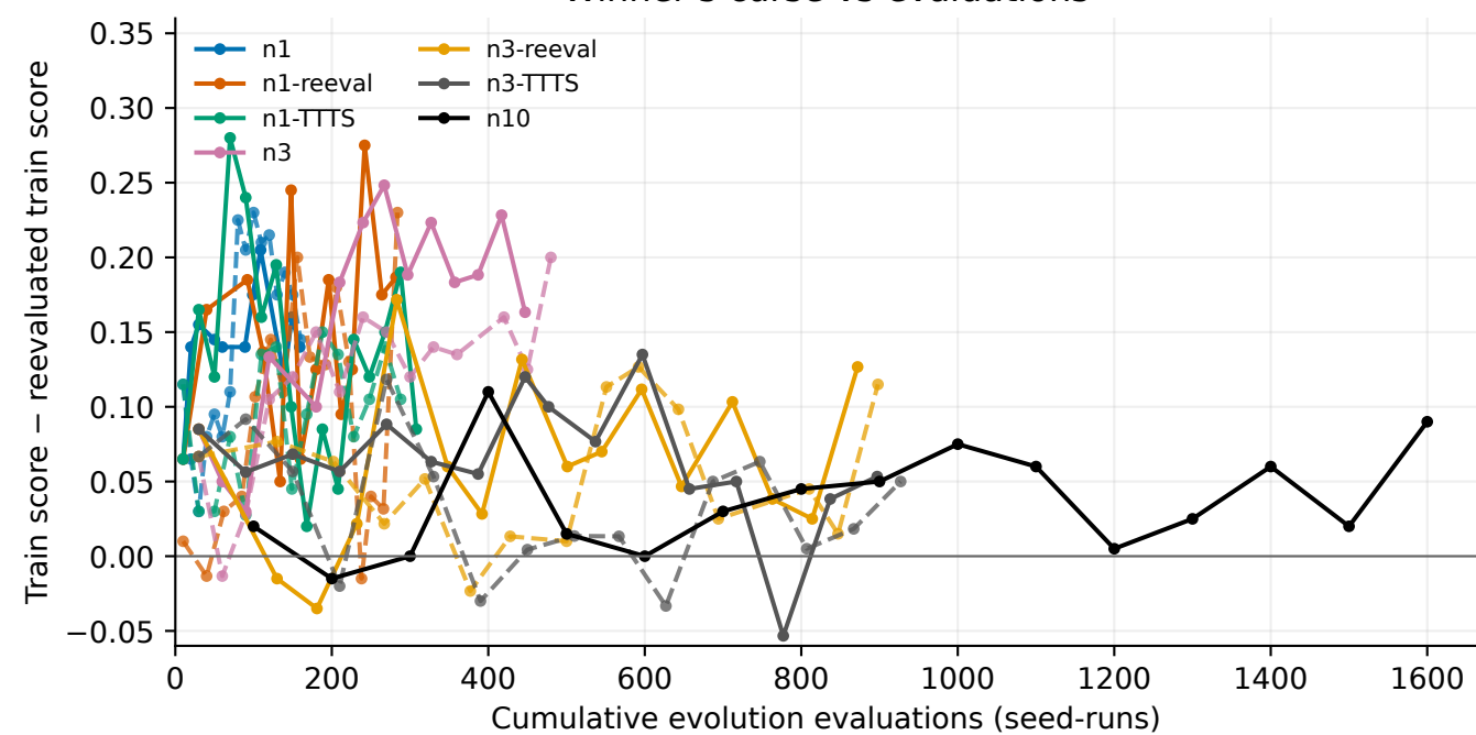
Winner's curse vs evaluations
