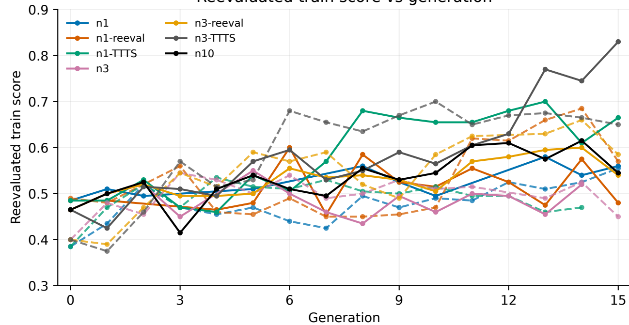
Reevaluated train score vs generation
