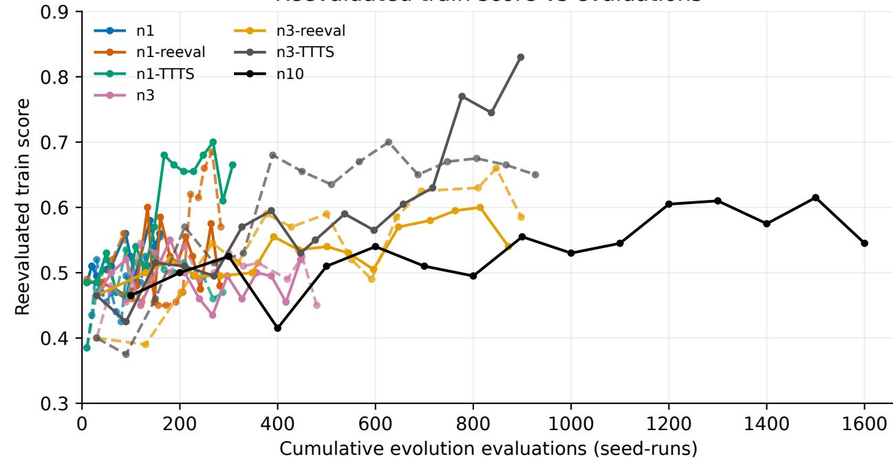
Reevaluated train score vs evaluations
