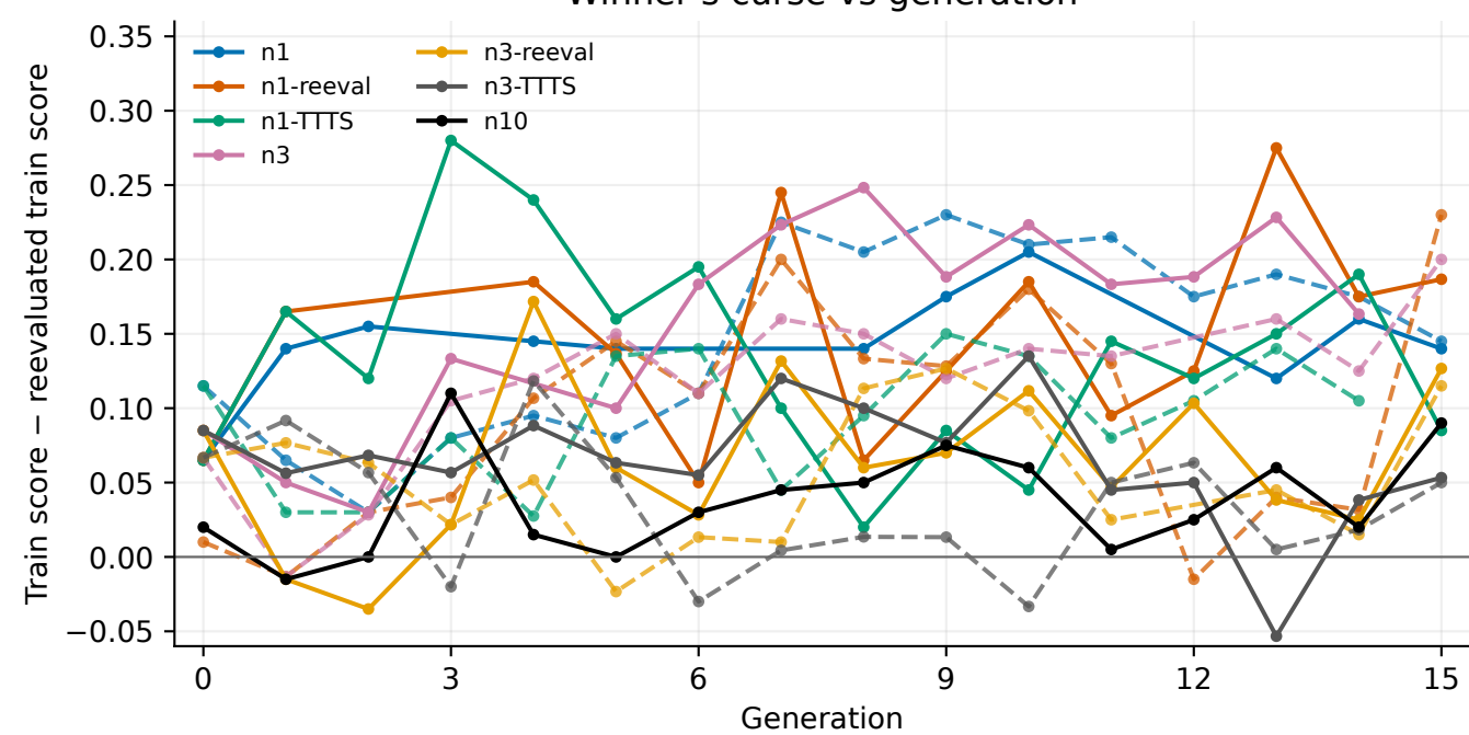
Winner's curse vs generation
