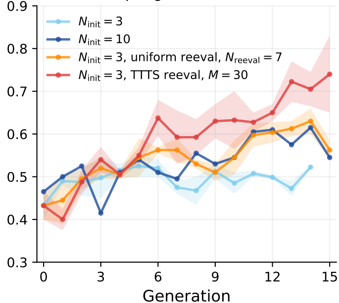
(a) Best offspring fitness (oracle)
