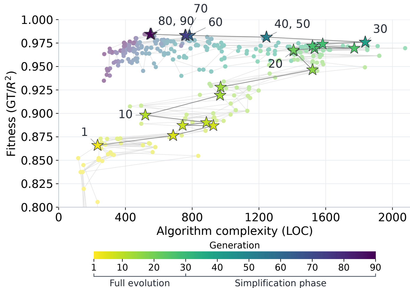
BasicSR evolution
