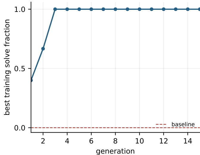
Run 708907 evolution trace
