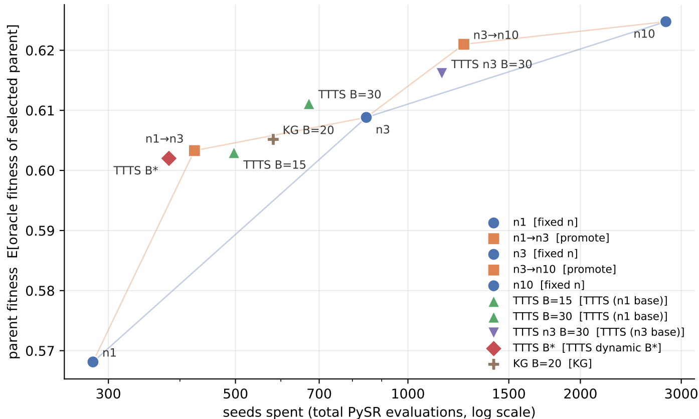
Reevaluation policies: fitness vs eval budget (oracle replay, runs 568245+568246 avg, final generation)
