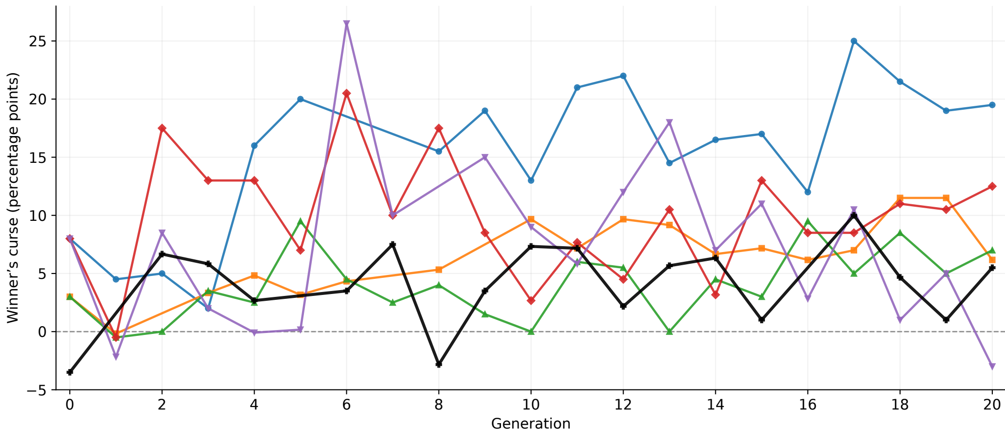
Winner's curse over evolution Train selection score – fresh-seed train reevaluation
