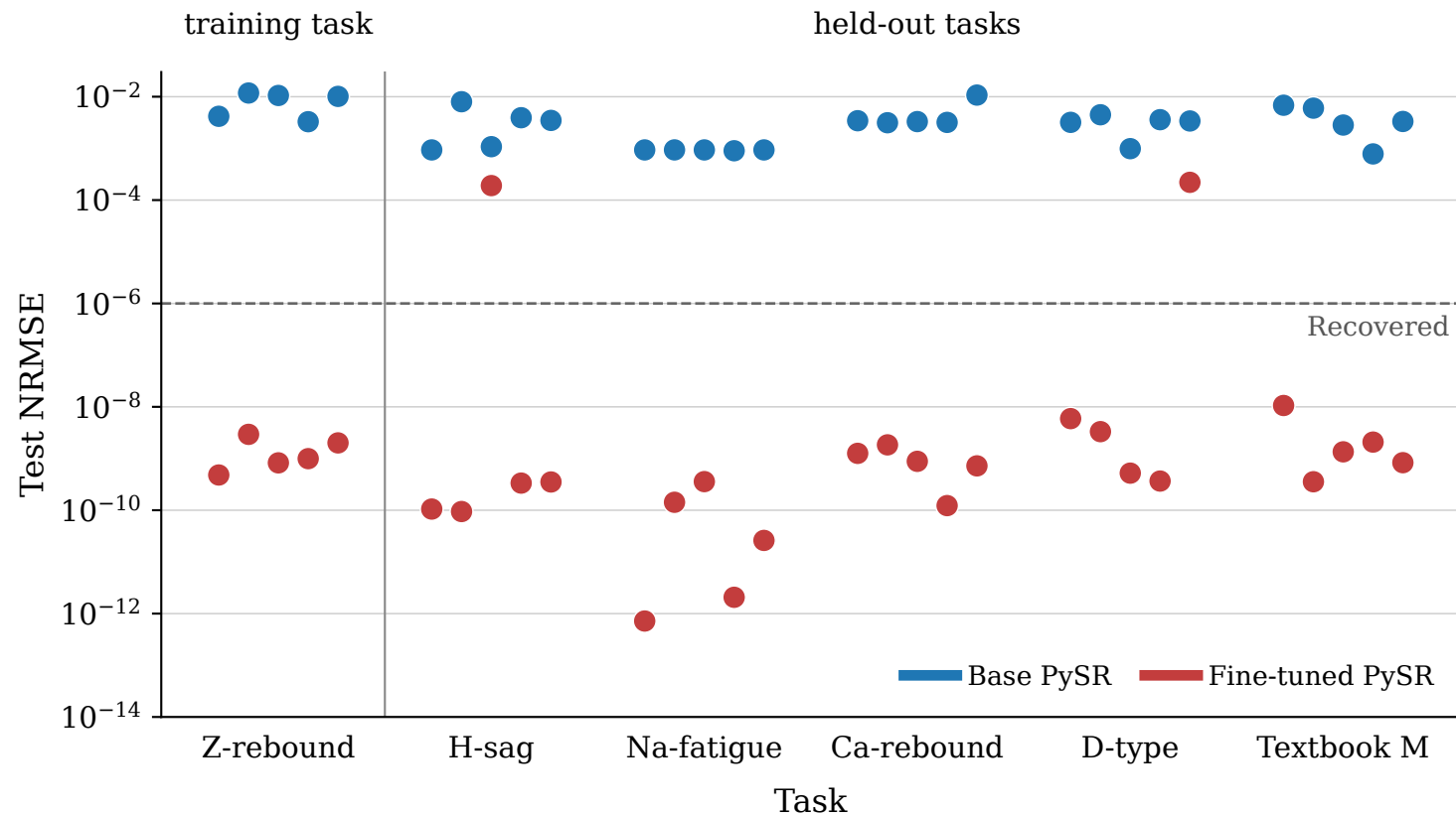
(a) NeuronBench
