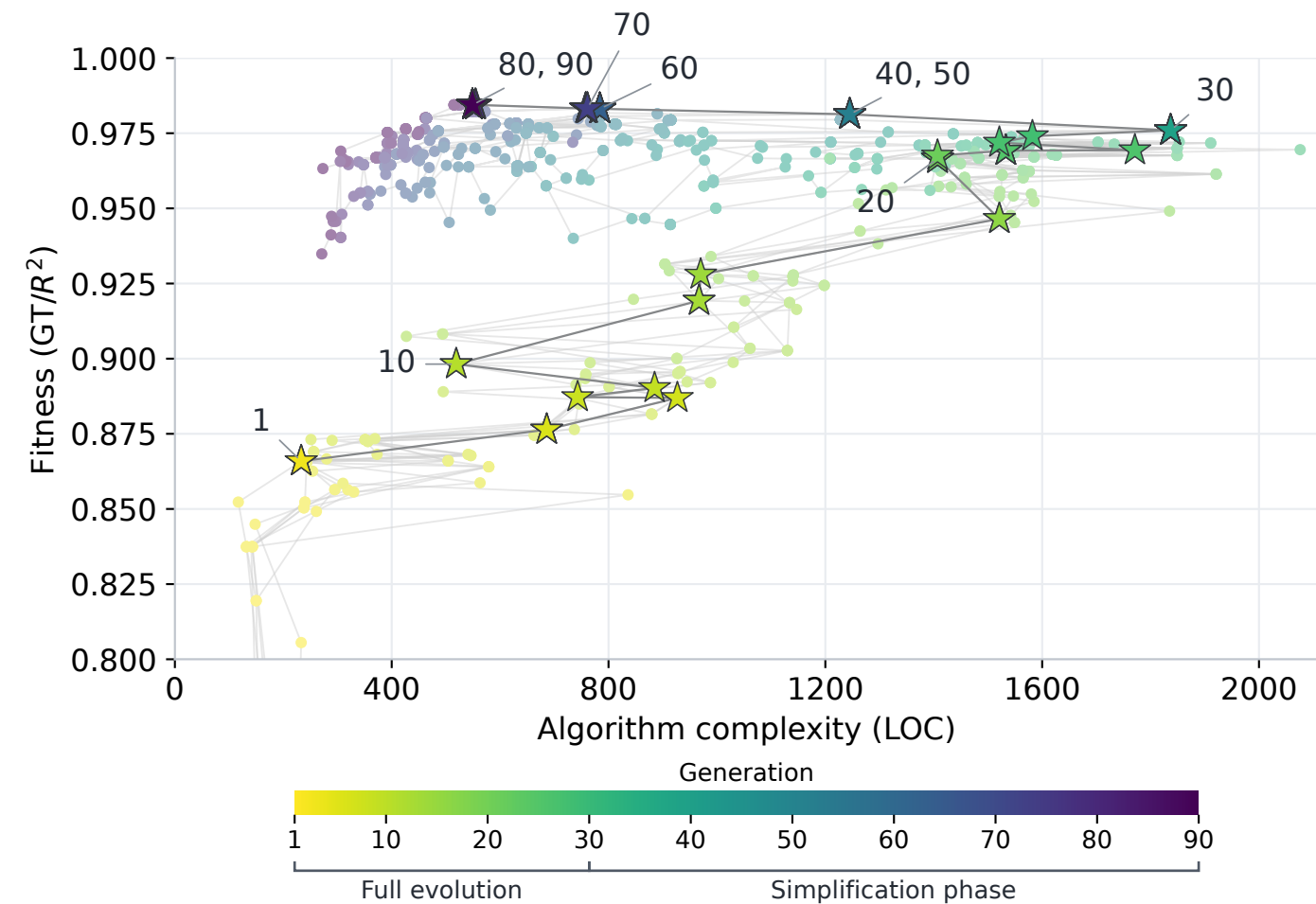
BasicSR evolution
