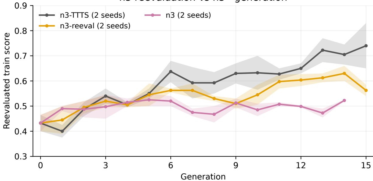
n3 reevaluation vs n3 · generation
