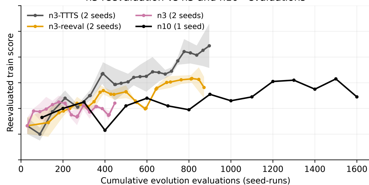
n3 reevaluation vs n3 and n10 · evaluations
