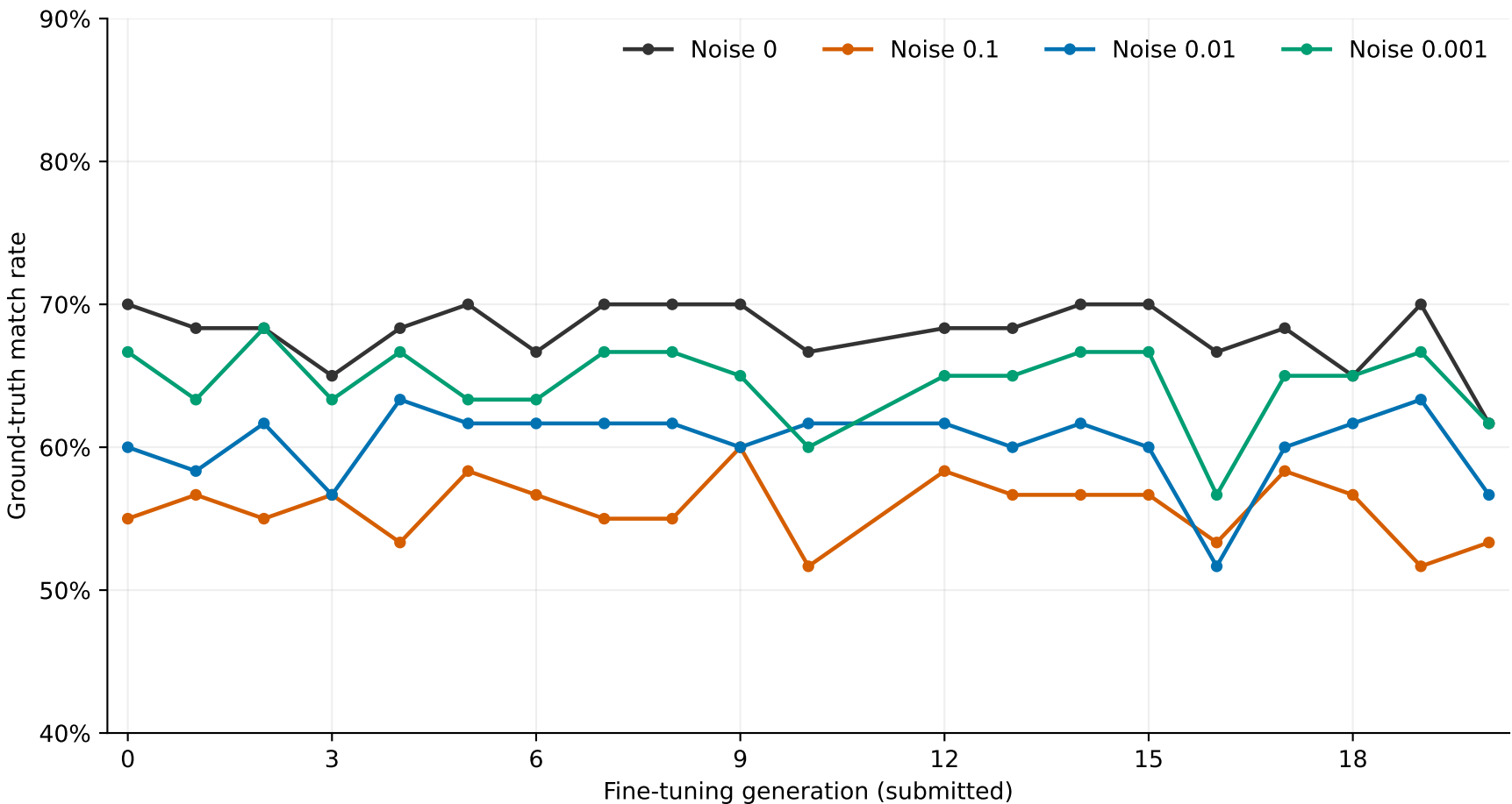
Run 140185 · Validation average GT Generation 0: checkpoint from 709715 · 20 datasets × 3 fresh seeds / noise
