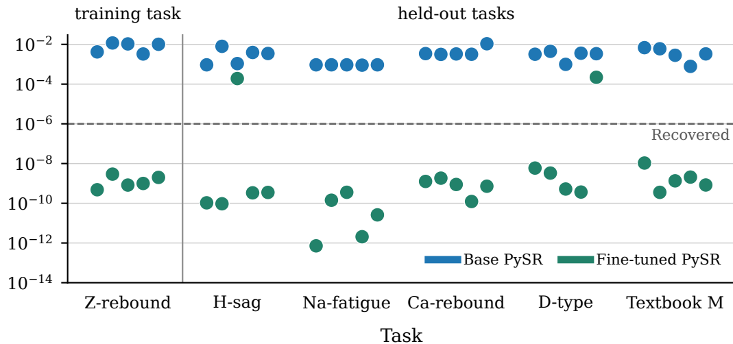
Test NRMSE
