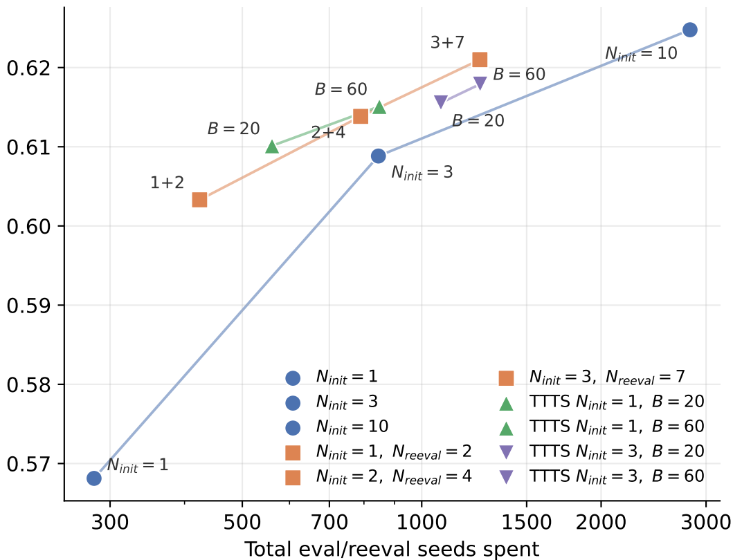
Expected true parent fitness
