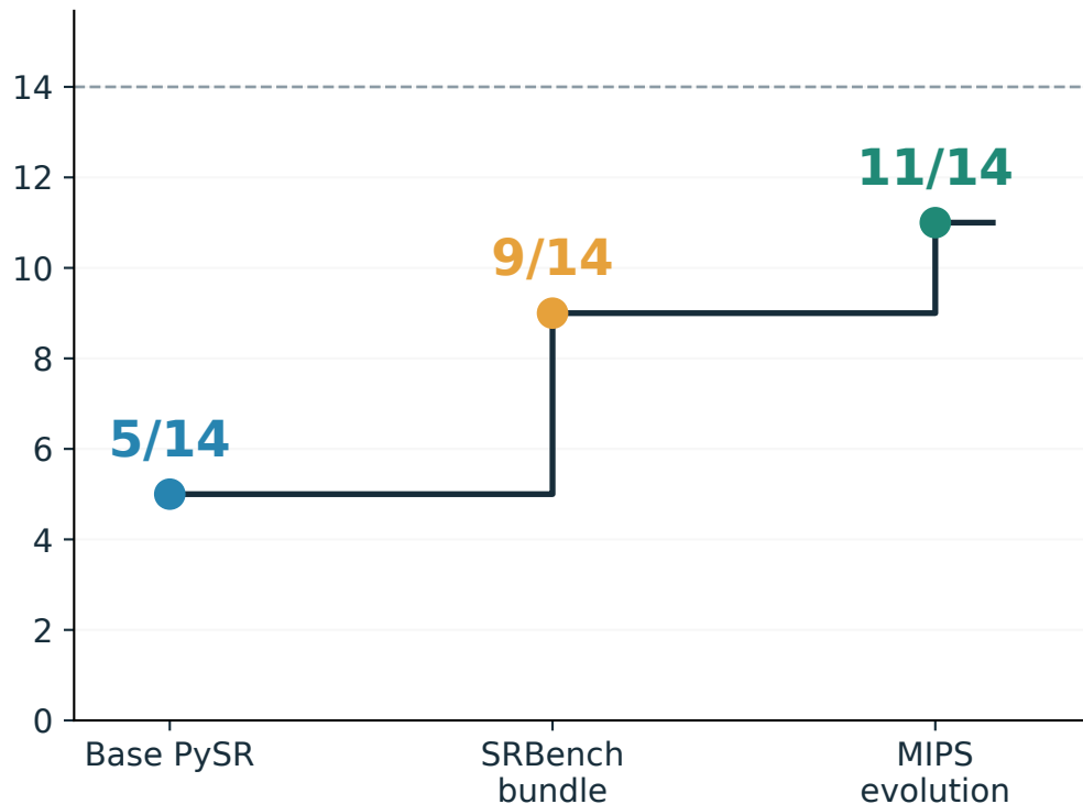
Previously unsolved overall problems
