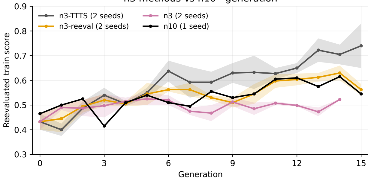
n3 methods vs n10 · generation
