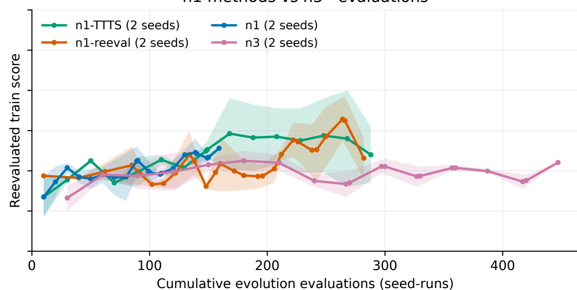
n1 methods vs n3 · evaluations
