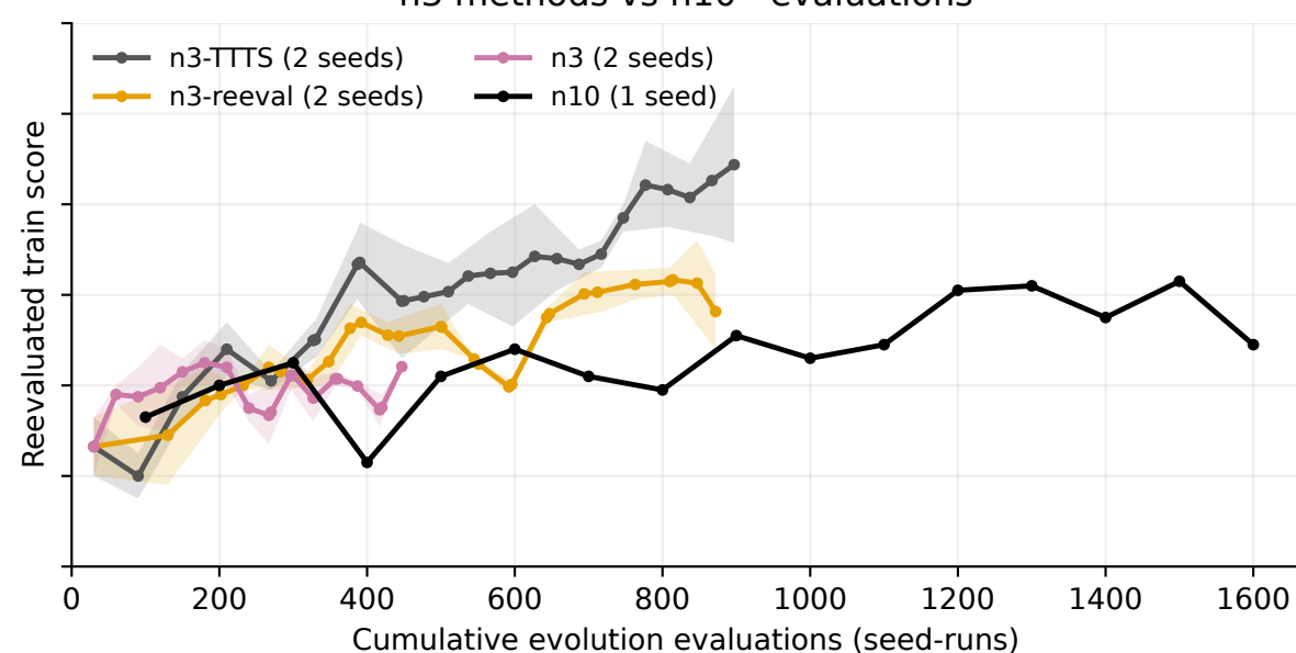
n3 methods vs n10 · evaluations
