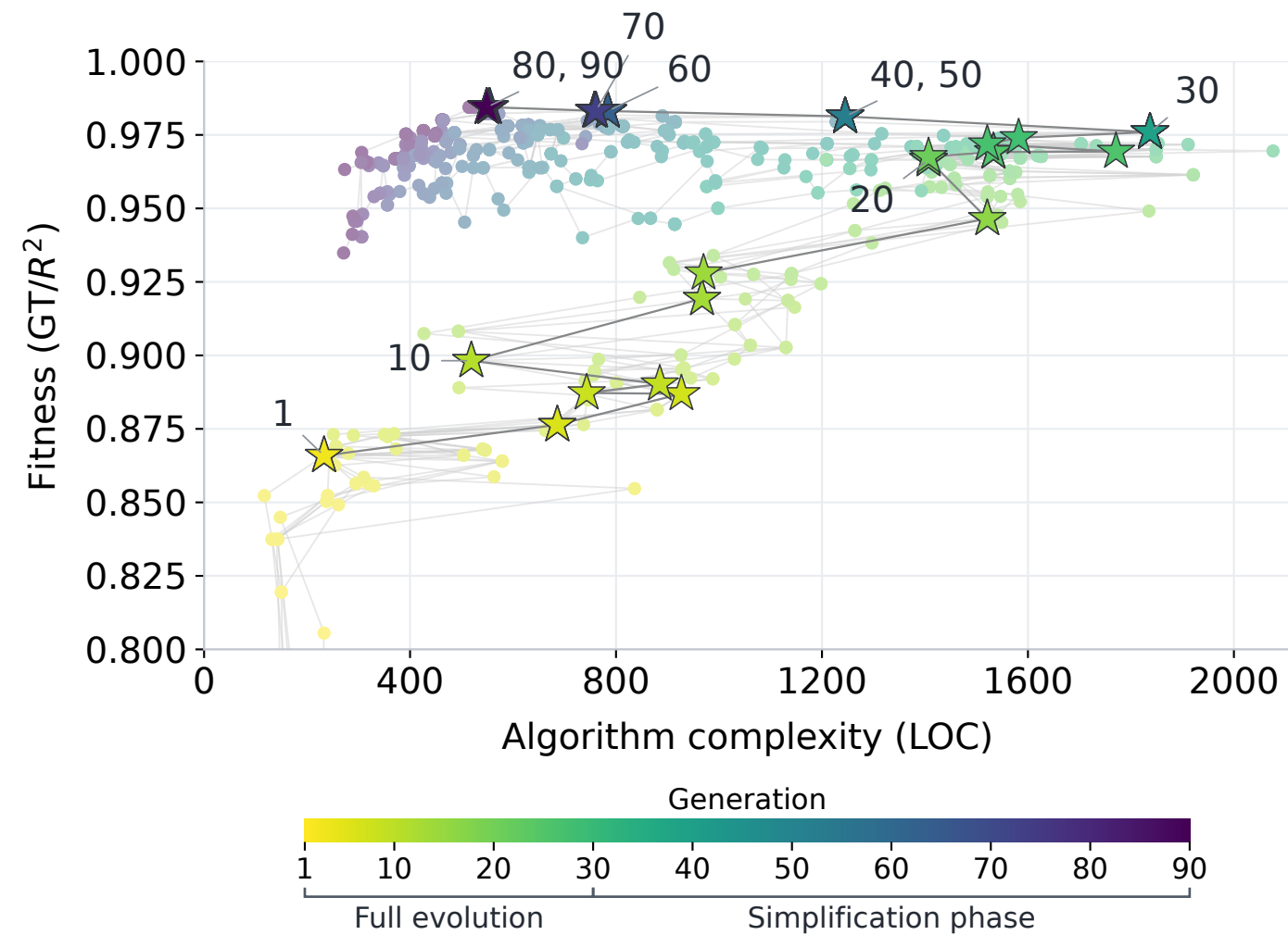
BasicSR evolution
