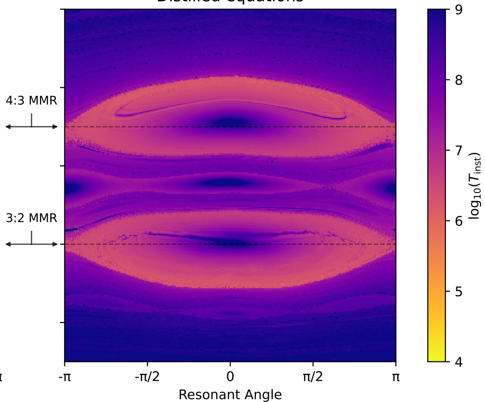
Distilled equations
