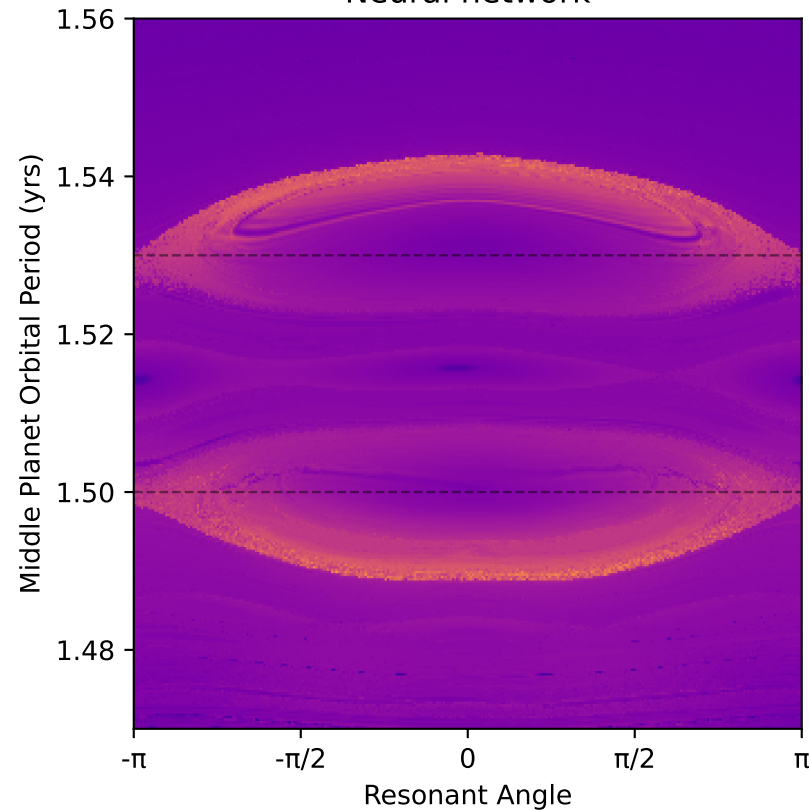
Neural network
