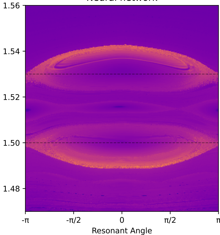
Neural network
