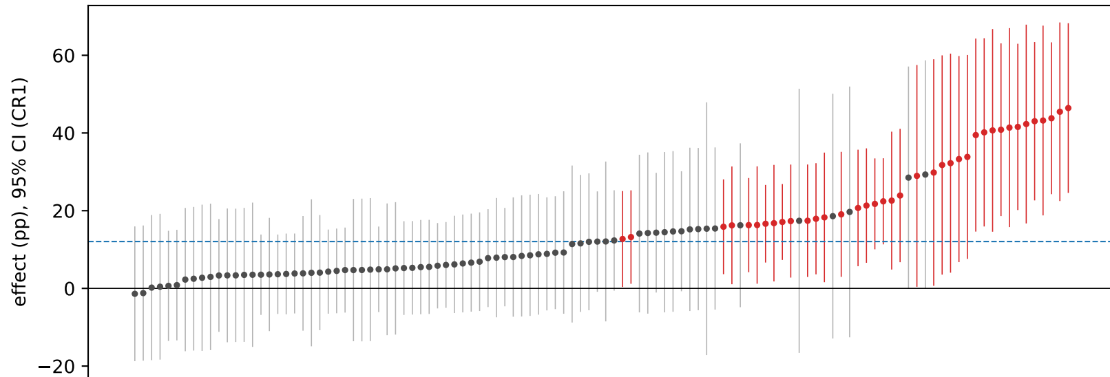
Specification curve — Non-Convention (primary); red = positive and p < 0.05
