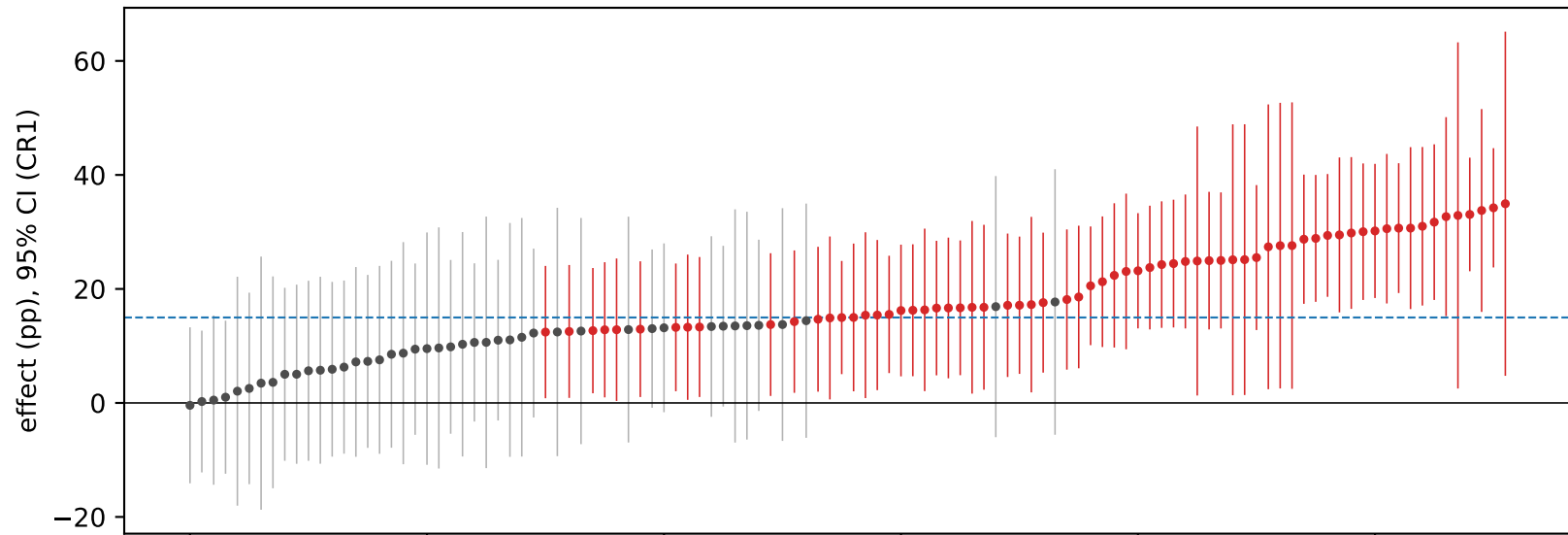
Specification curve — UNCITRAL (secondary); red = positive and p < 0.05
