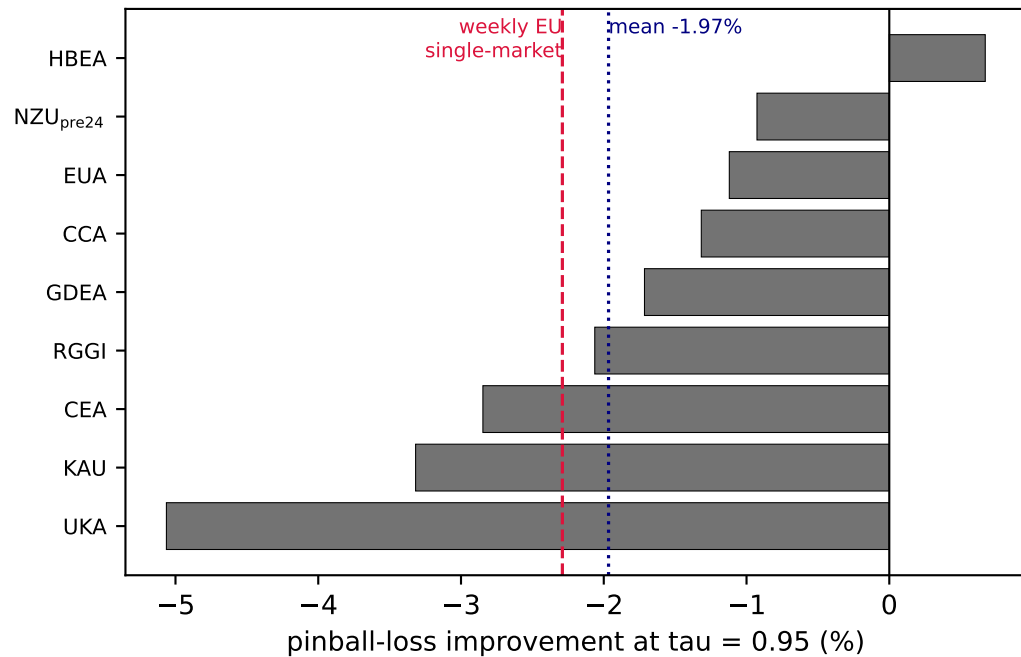
(b) Upper-tail gain: the dimensionality penalty
