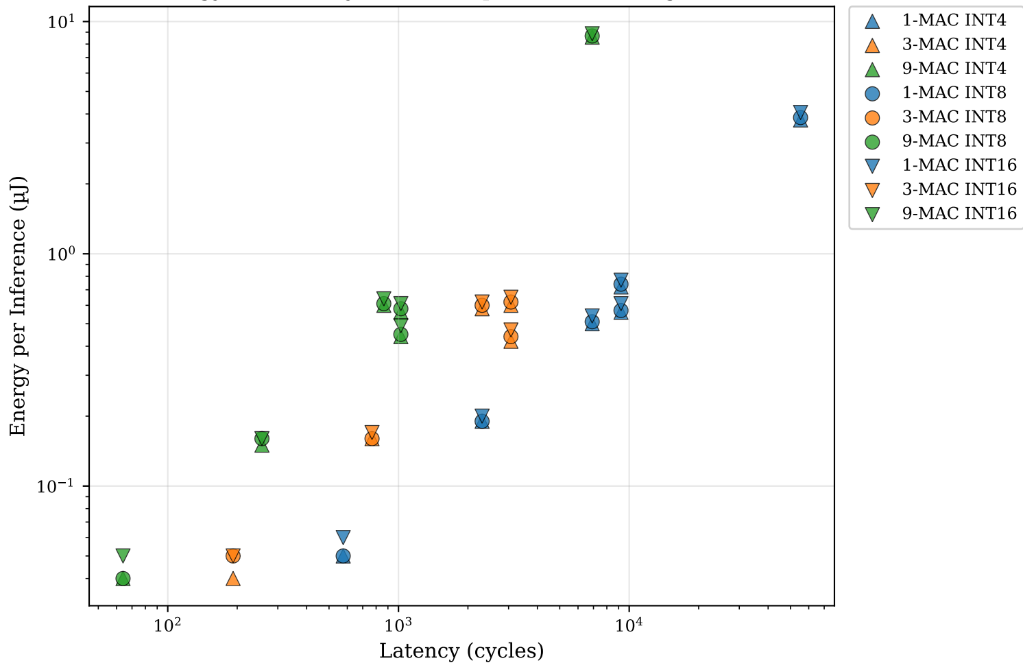
Energy vs. Latency — Timeloop DSE (All Configurations)
