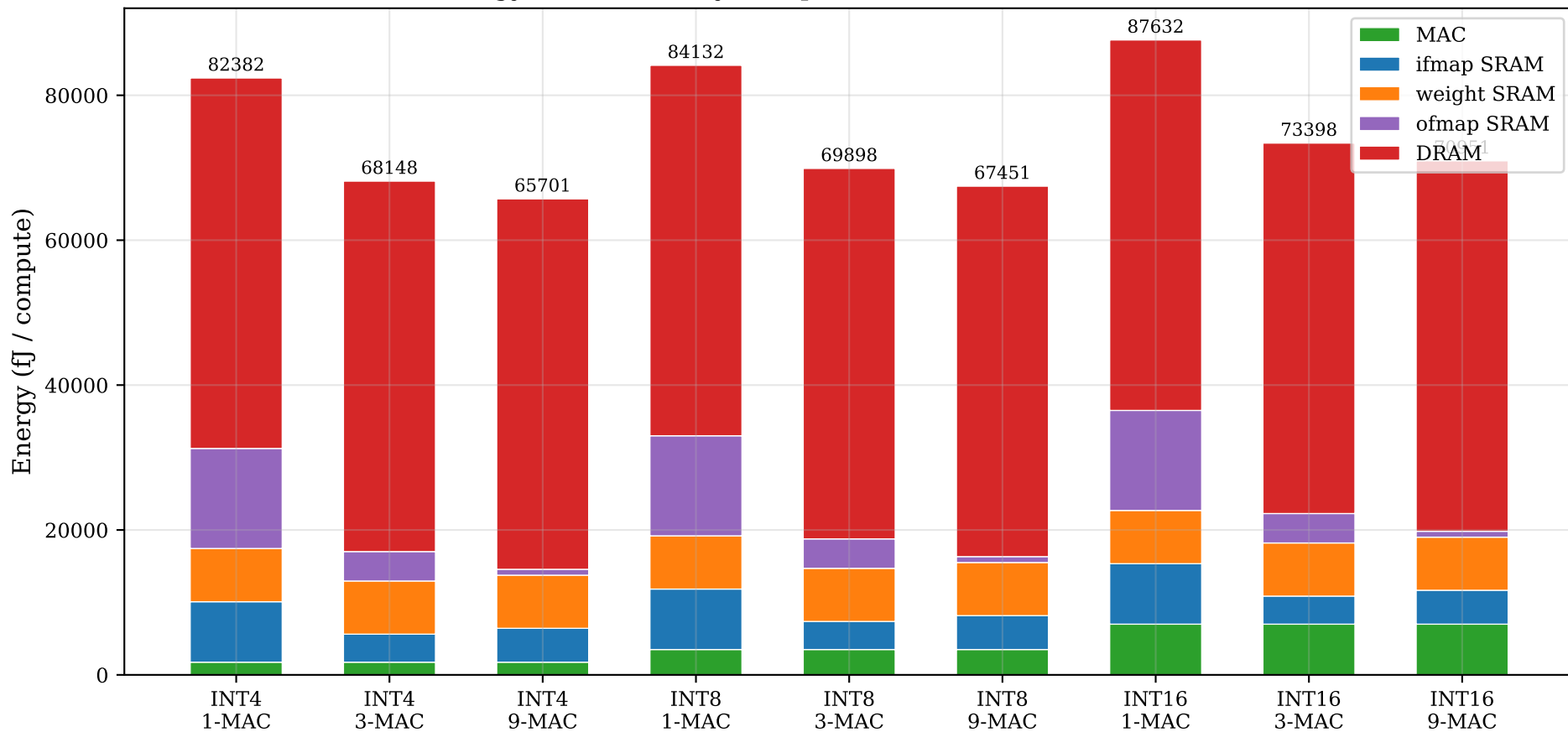
Energy Breakdown by Component — Conv2D 16×16 Baseline
