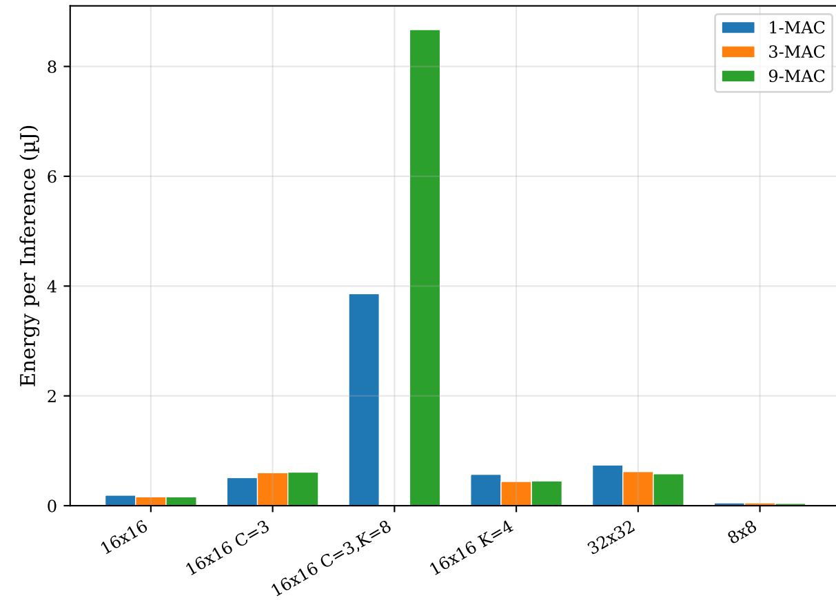
Energy vs. Problem Size (INT8)
