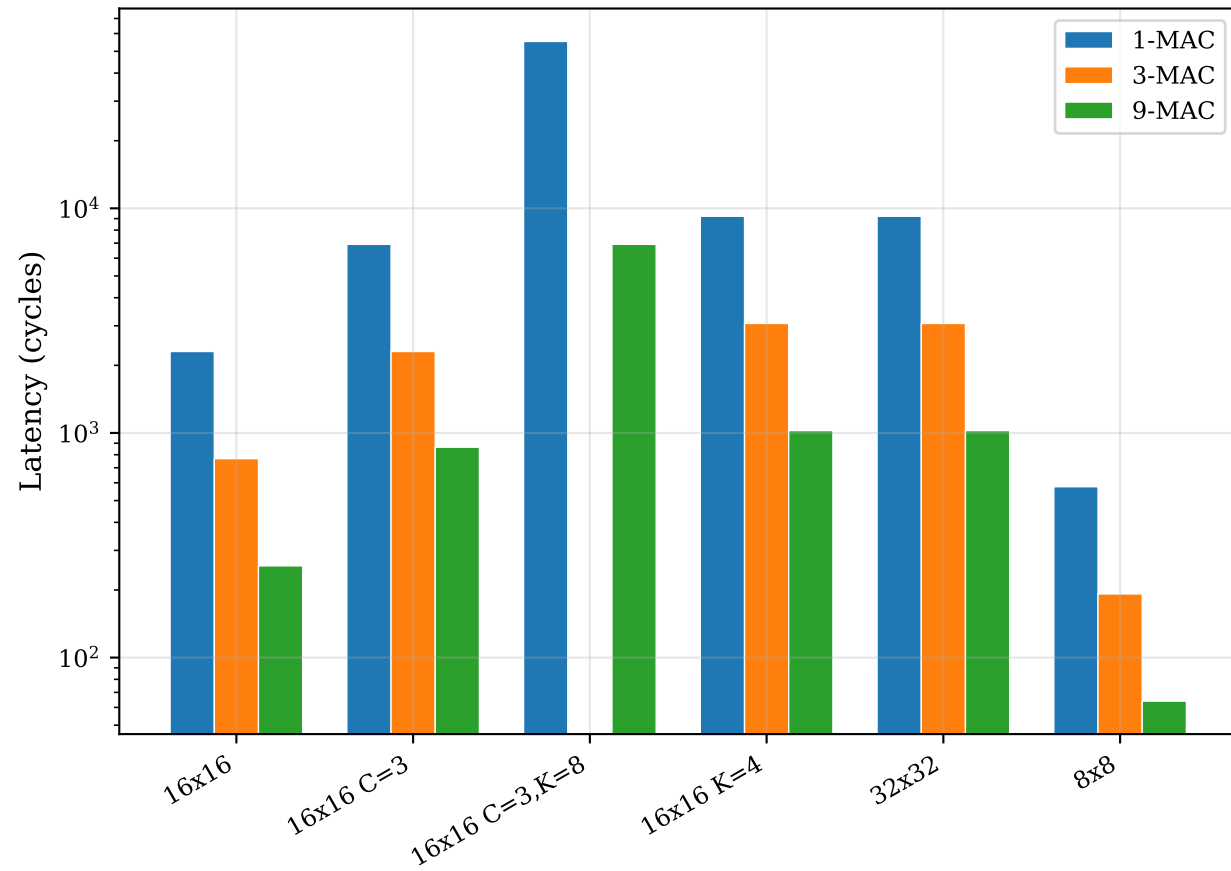
Latency vs. Problem Size (INT8)
