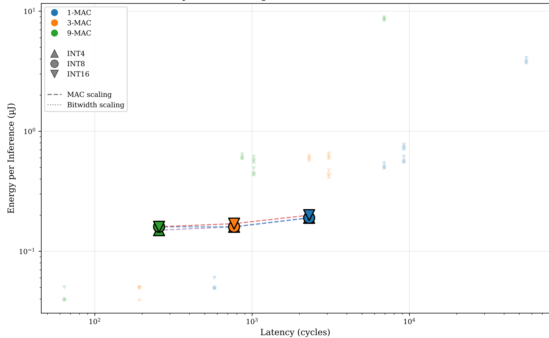
Timeloop DSE — 9 Configurations Selected for FPGA Validation
