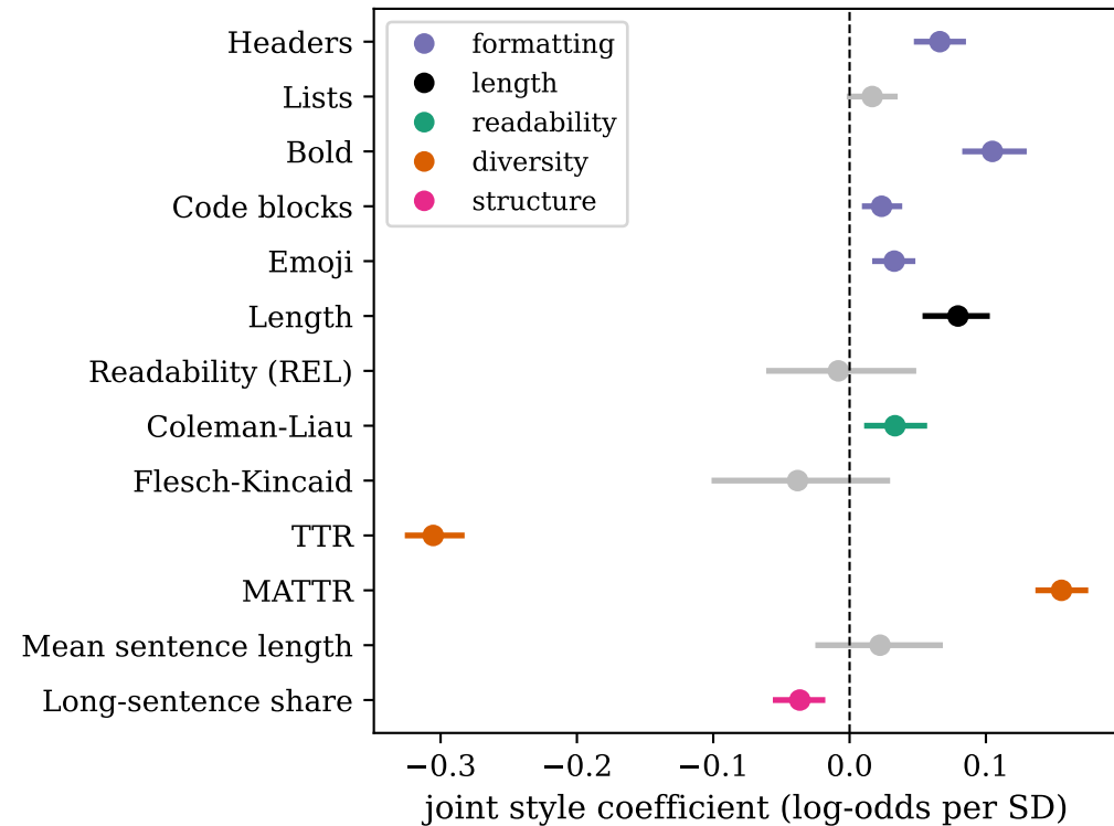
Joint model: what moves a vote (95% CI, BH-corrected; grey = n.s.)
