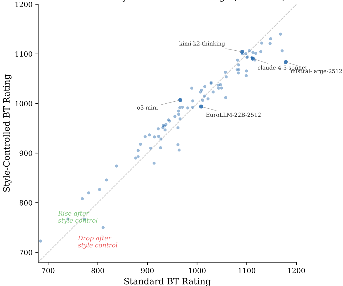
Standard vs. Style-Controlled Ratings ( r = 0.976 )
