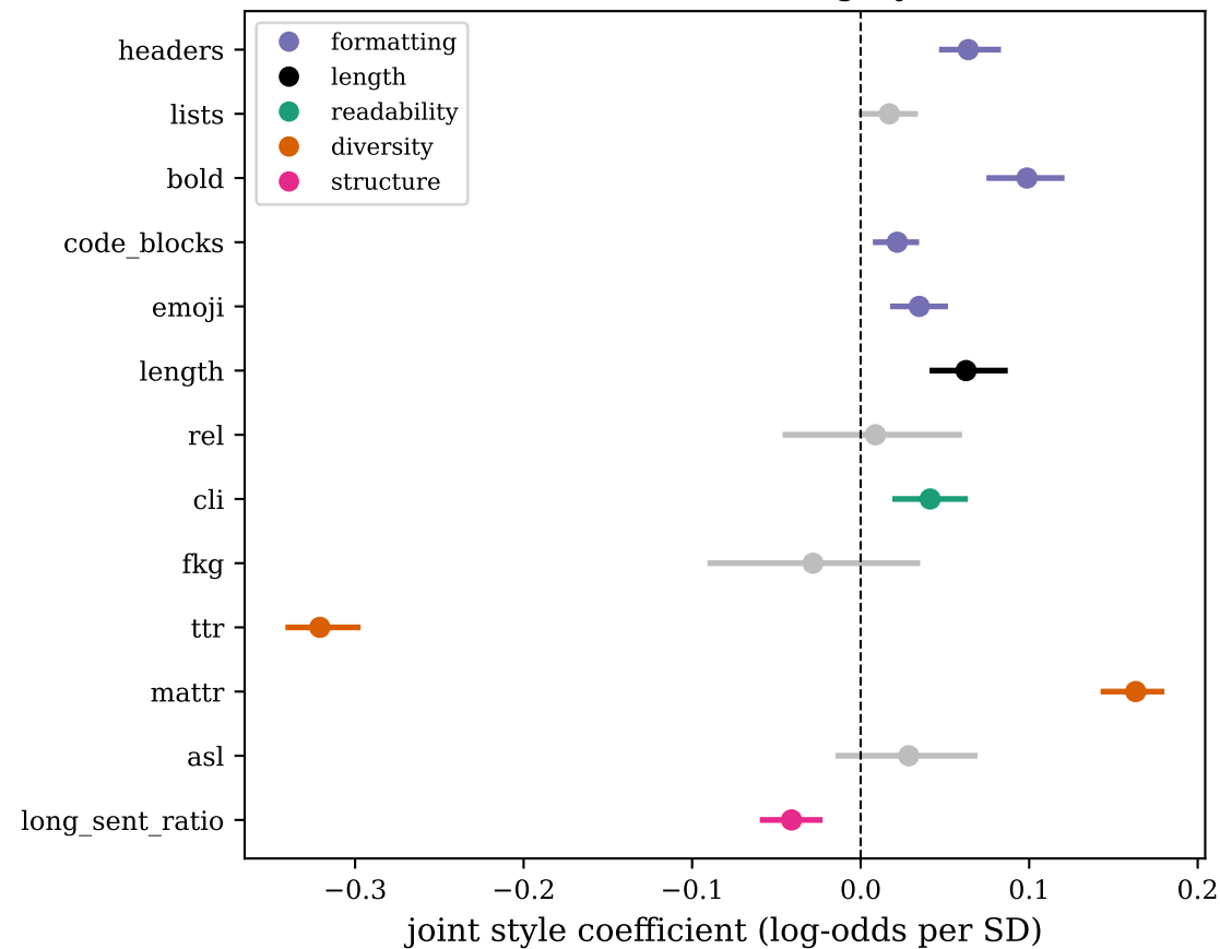
Joint model: what moves a vote (95% CI, BH-corrected; grey = n.s.)
