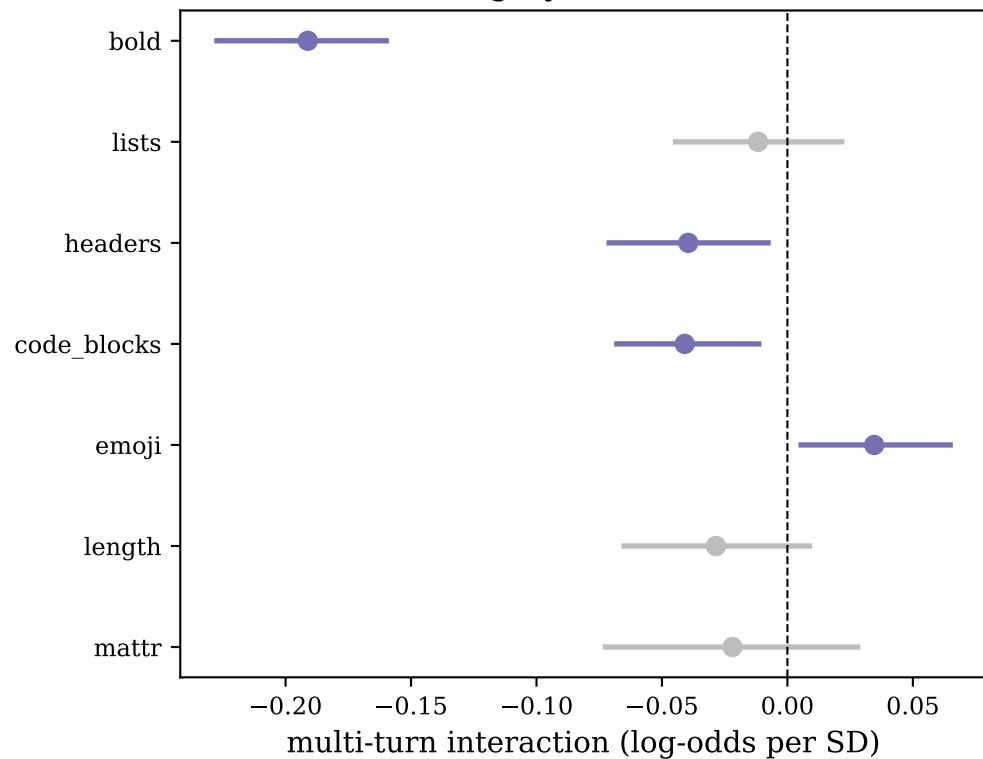
Interaction with vote-time conversation depth (95% CI; grey = n.s. after BH)
