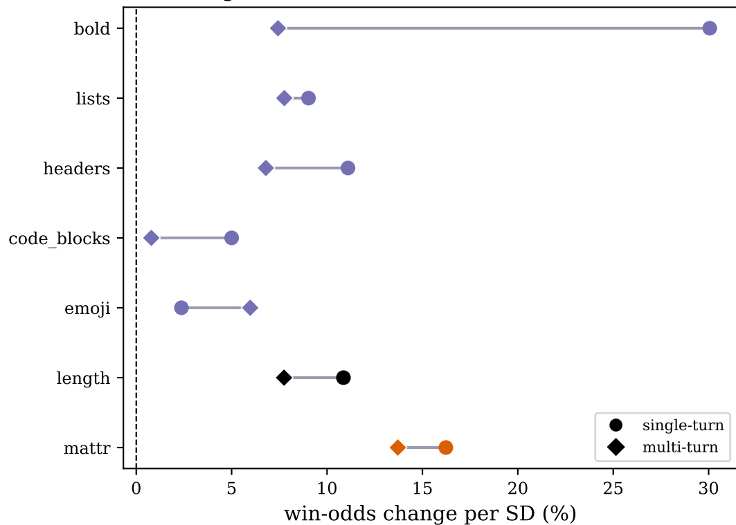
Depth visible at the vote single-turn (circle) vs multi-turn (diamond)
