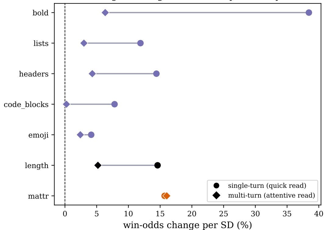
Single-turn (circle) vs multi-turn (diamond) formatting and length shrink, only diversity holds
