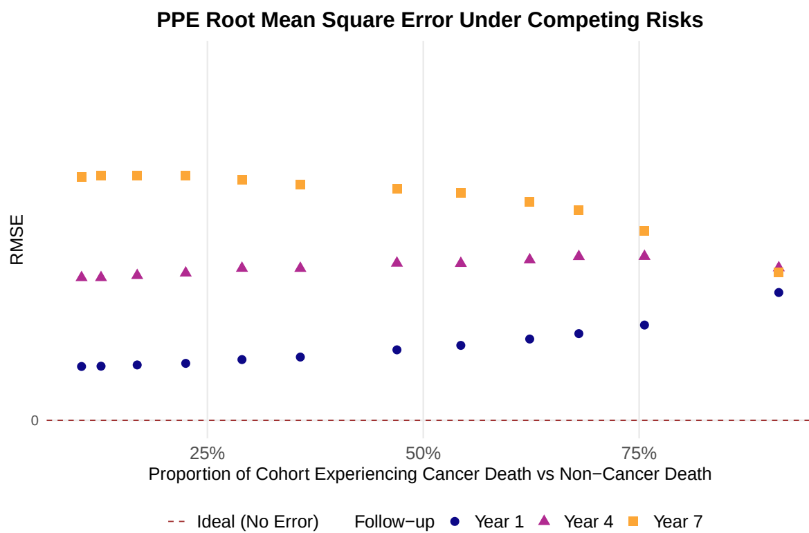
Figure 4: PPE root mean square error under competing risks.
