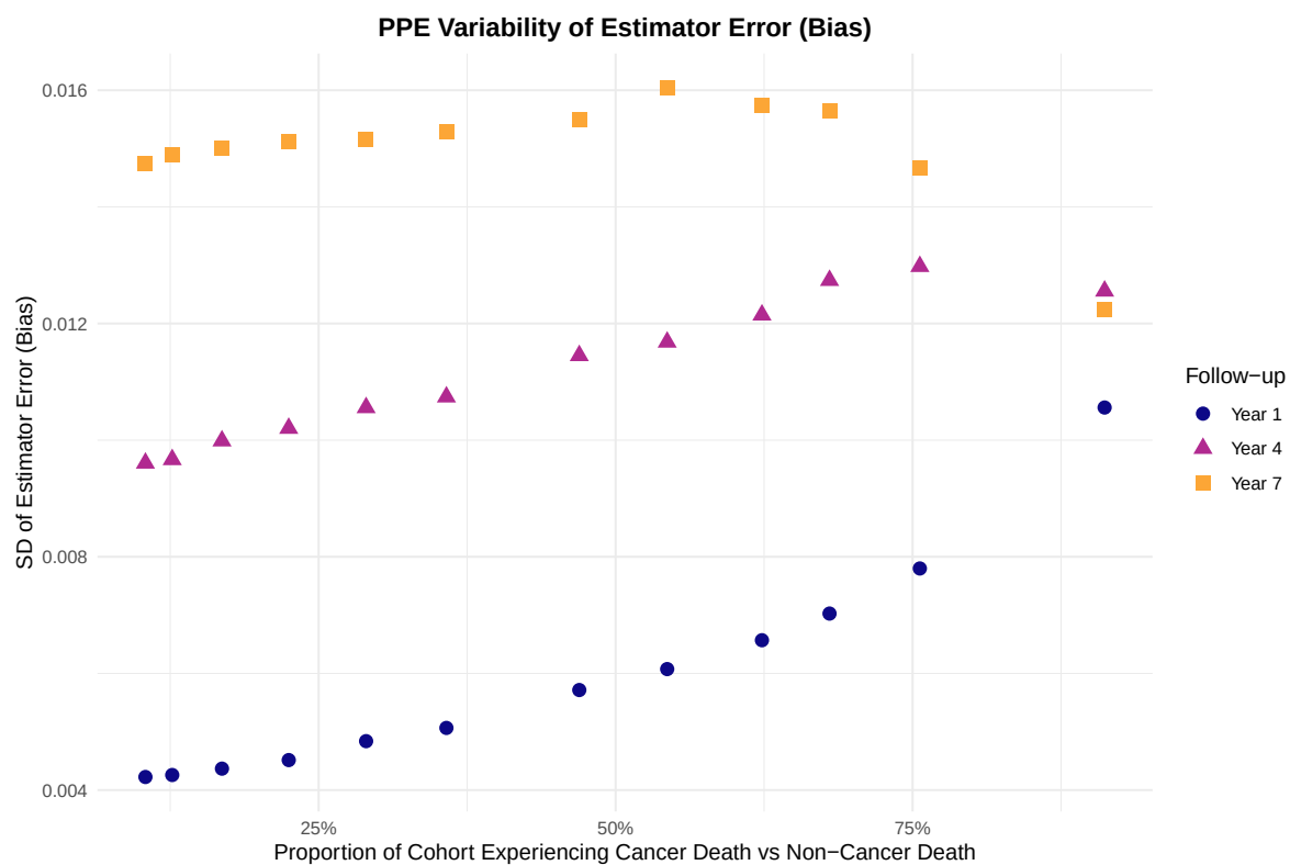
Figure 6: PPE empirical dispersion under competing risks.
