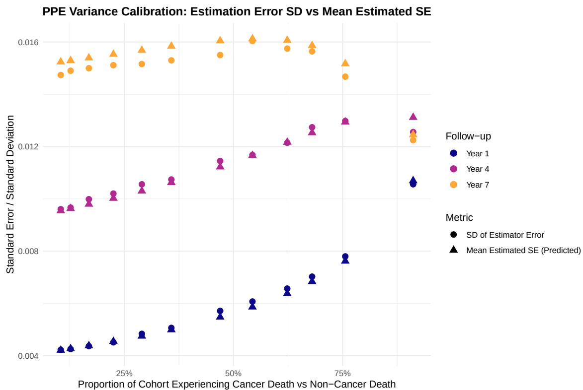
Figure 8: Direct comparison of true empirical dispersion versus mean estimated SE.
