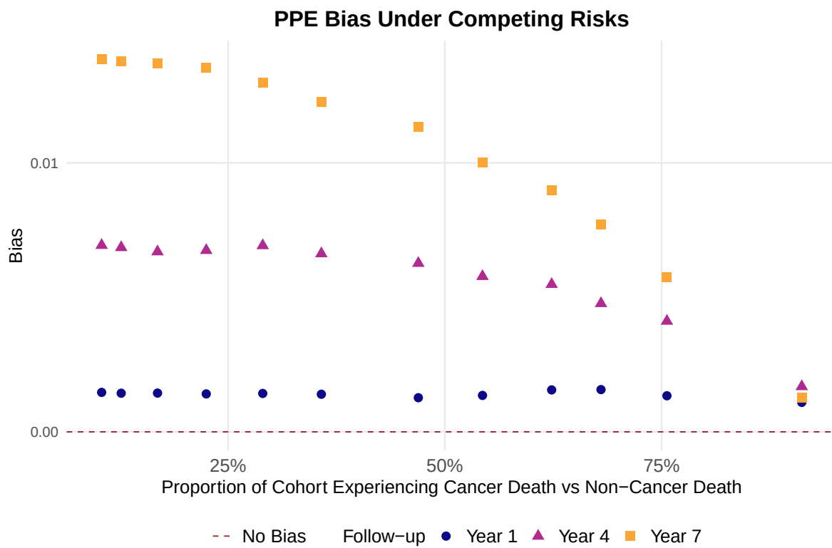
Figure 3: PPE bias under competing risks.
