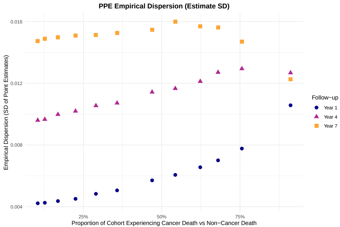
Figure 5: PPE empirical dispersion under competing risks.
