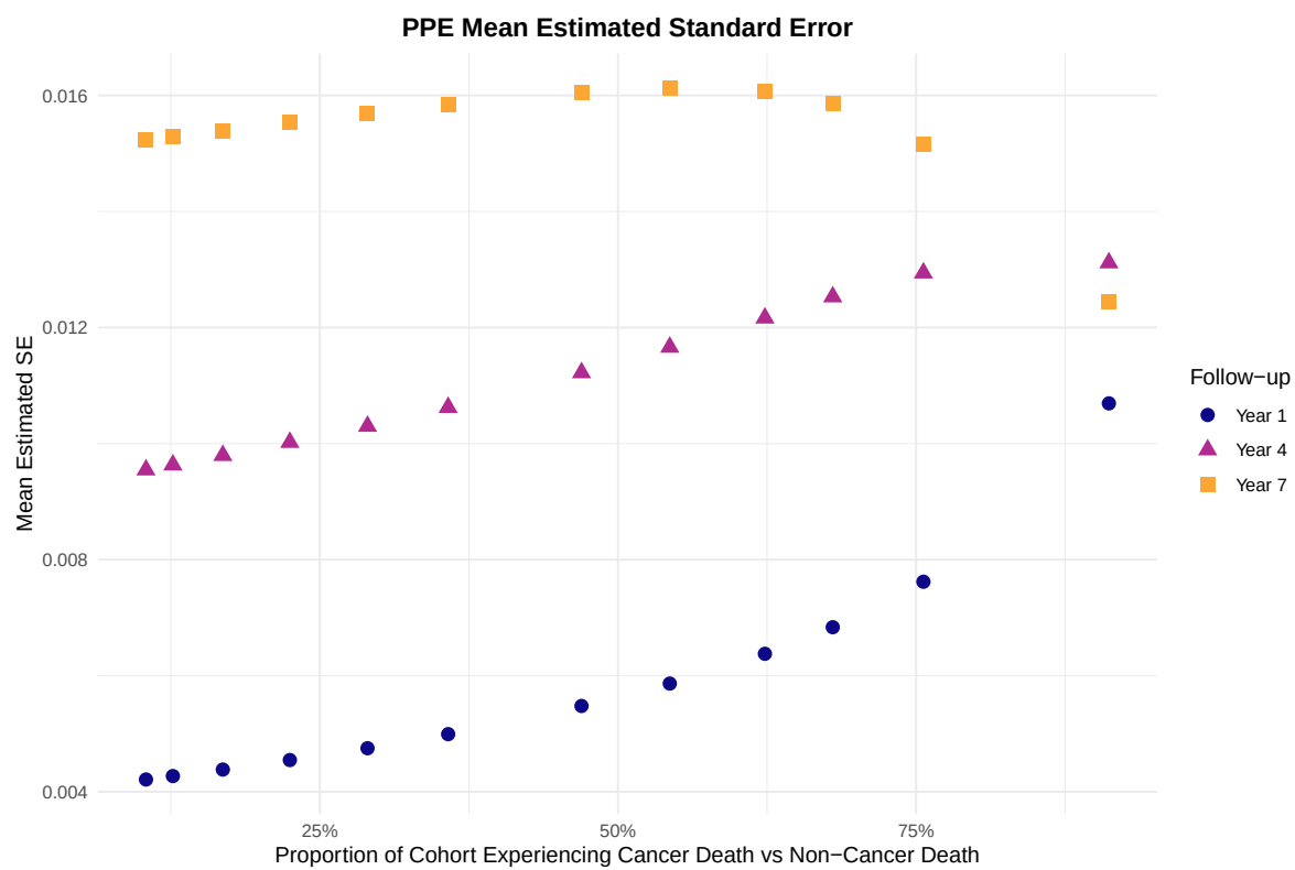
Figure 7: PPE mean estimated standard error under competing risks.
