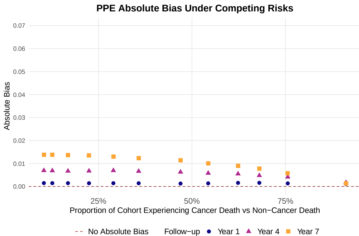
Figure 2: PPE bias under competing risks.
