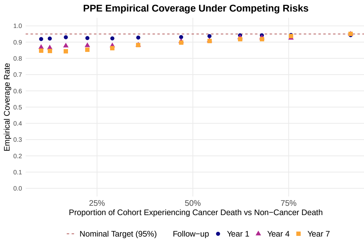
Figure 1: PPE empirical coverage under competing risks.
