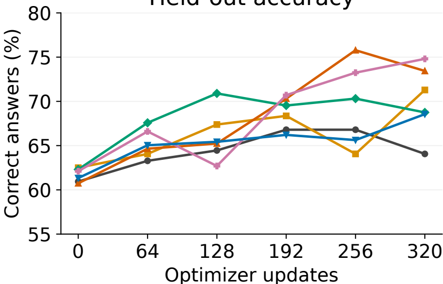
Held-out accuracy
