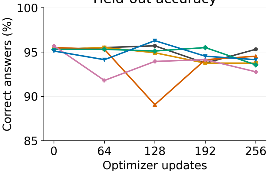
Held-out accuracy
