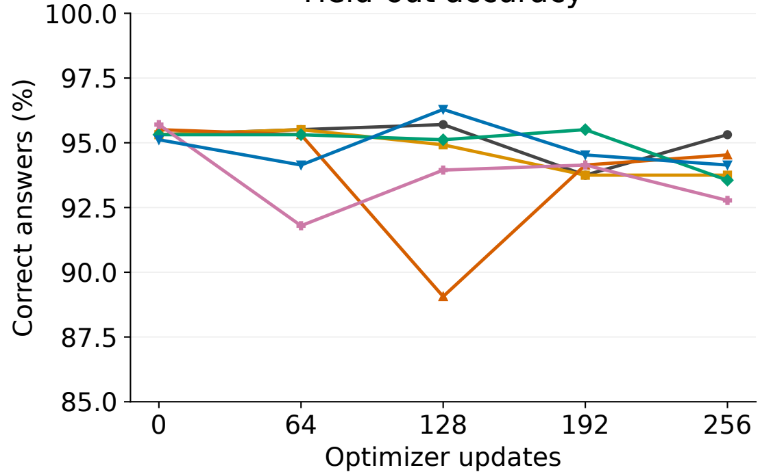
Held-out accuracy
