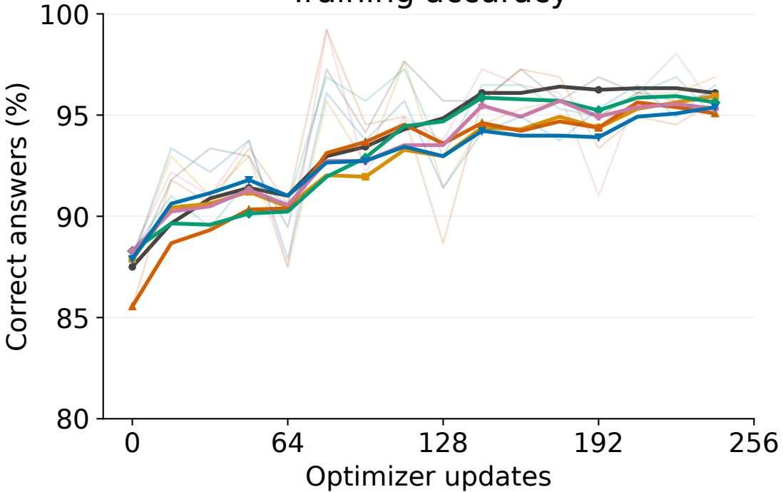
Training accuracy
