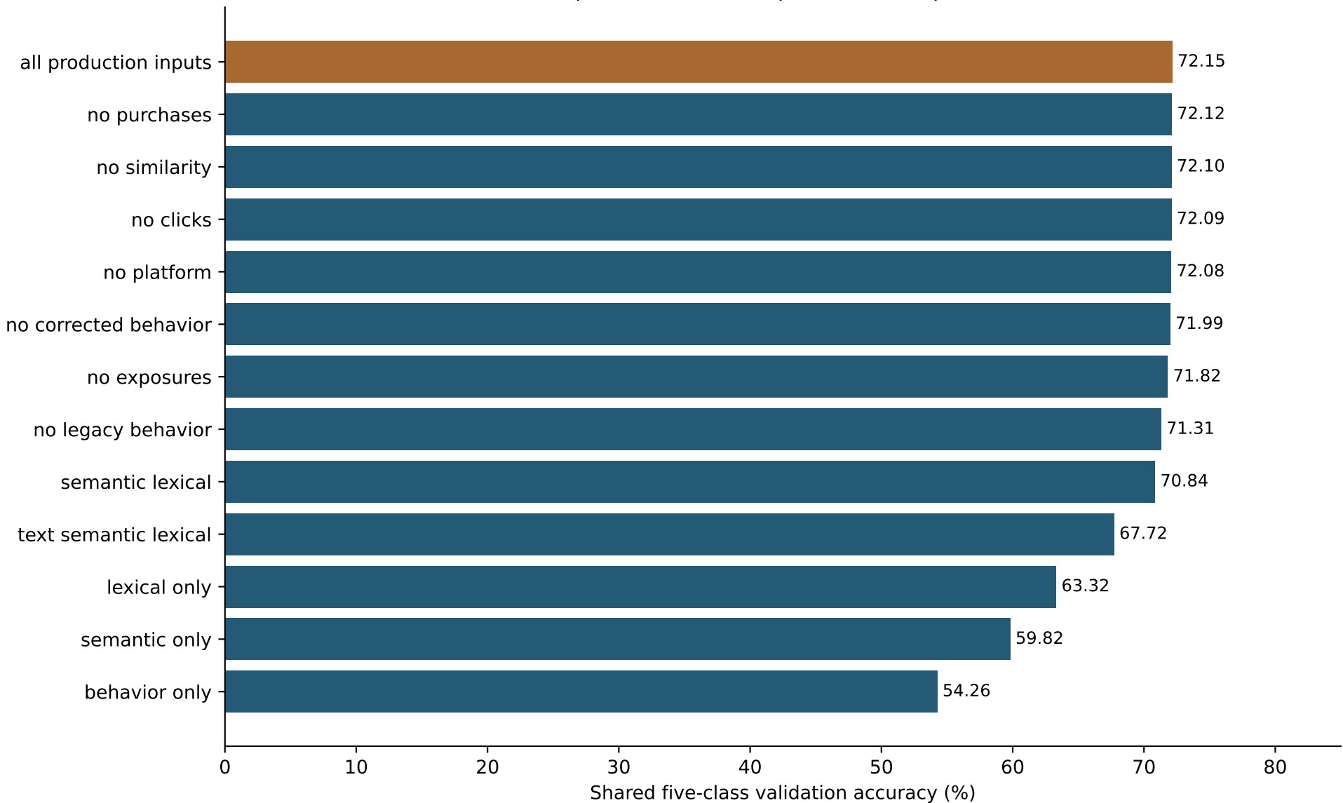
Retrained input ablations: 2M pairs, 2,510 updates, seed 173
