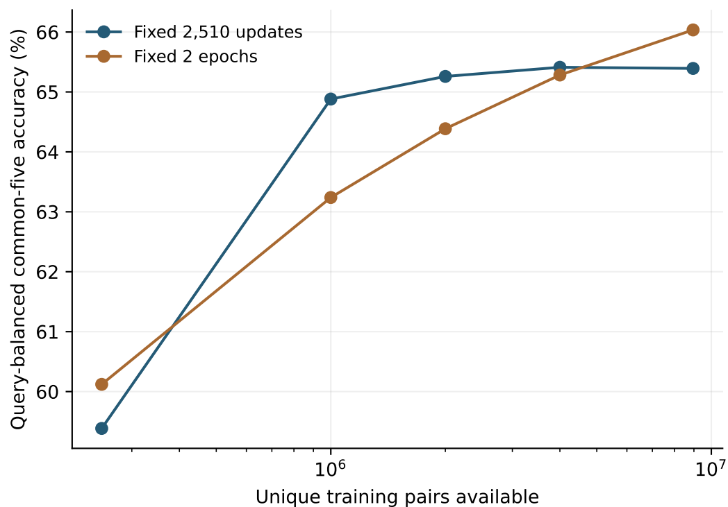
Data scaling: production-size feature model, seed 173
