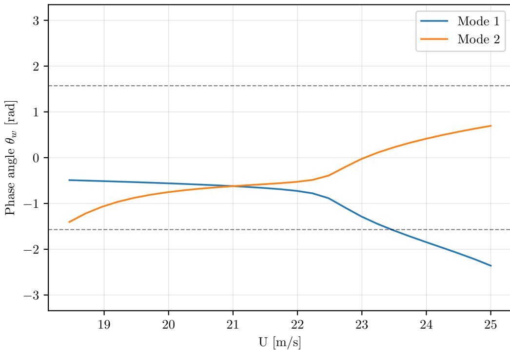
Phase angle \theta_w by which the bending part leads the torsion part
