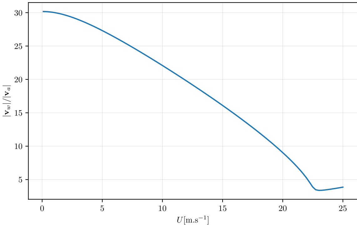
Relative bending-torsion contribution ( |\mathbf{v}_w|/|\mathbf{v}_a| ) - Mode 1
