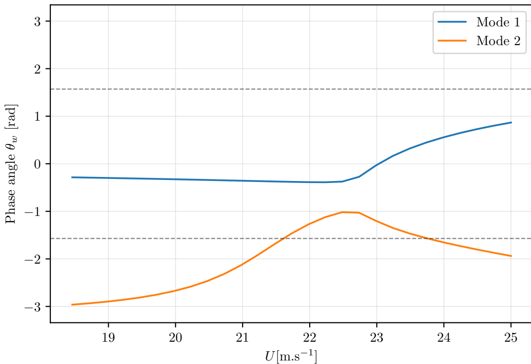
Phase angle \theta_w by which the bending part leads the torsion part
