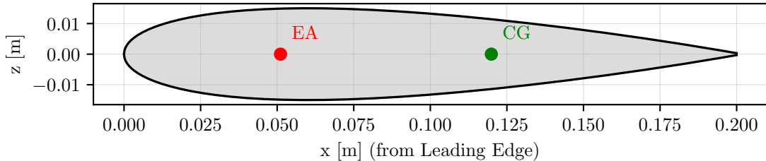
NACA0015 section ( c = 0.2 m)
