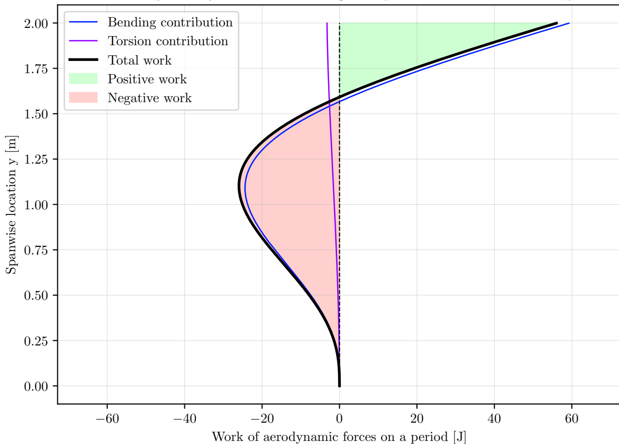
Work done by aerodynamic forces along the span at U = 25\text{m.s}^{-1} on a period
