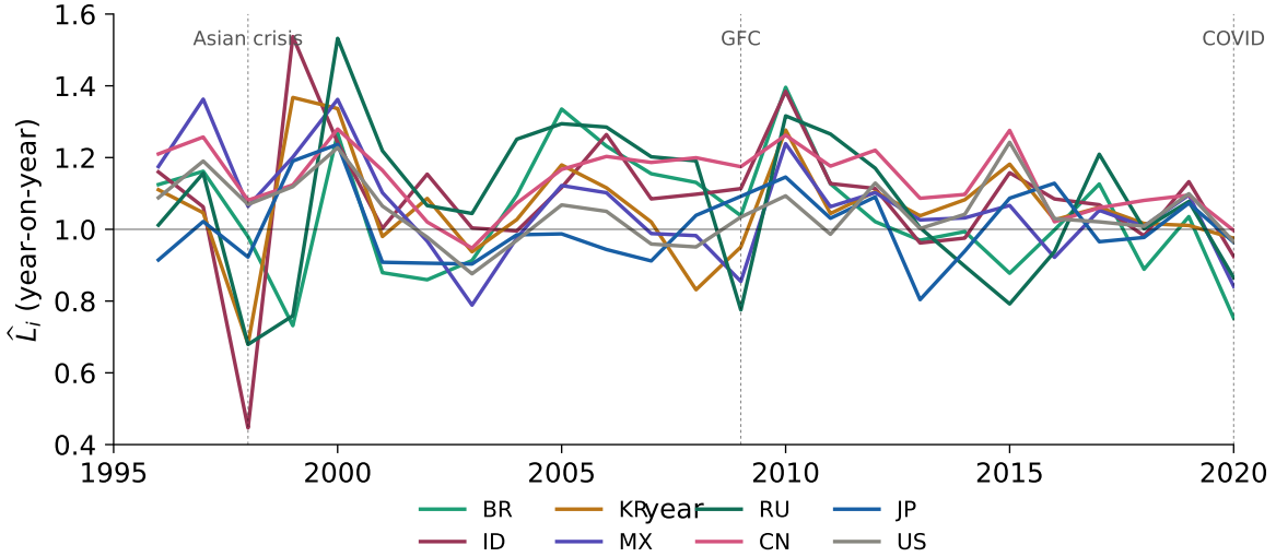
Figure 1: Labor-endowment hats pick up every major macro shock. Year-on-year labor-endowment hat \hat{L}_i for selected countries, recovered from the cost-share identity that pins L_i each year. Dashed vertical lines mark the three benchmark events in the panel: the 1997–98 Asian financial crisis ( \hat{L}_{ID} = 0.45 , \hat{L}_{KR} = 0.68 ); the 2008–09 Global Financial Crisis ( \hat{L}_{RU} = 0.78 , \hat{L}_{MX} = 0.86 , while emerging Asia keeps growing); and the 2019–20 COVID-19 disruption ( \hat{L}_{BR} = 0.75 , \hat{L}_{MX} = 0.84 , with East Asia largely shielded).
