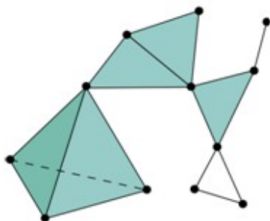
Simplicial complex
