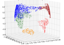
Sphere: 3023 points
