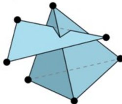
Invalid Simplicial complex
