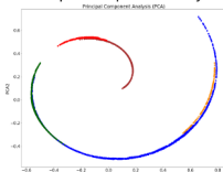
Principal Component Analysis
