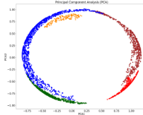
Sphere: 3023 points
