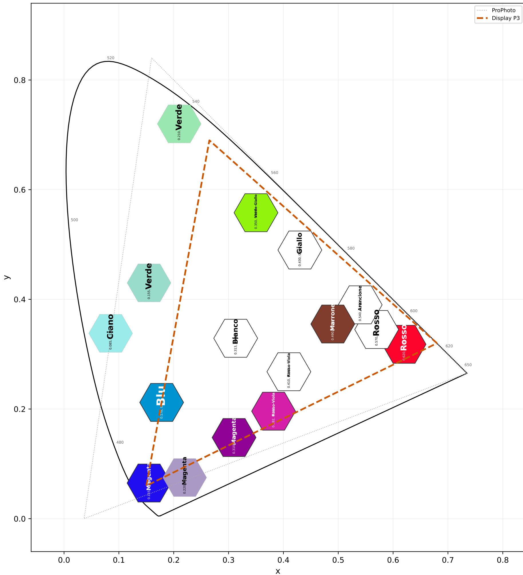
CIE 1931 — Display P3 gamut
