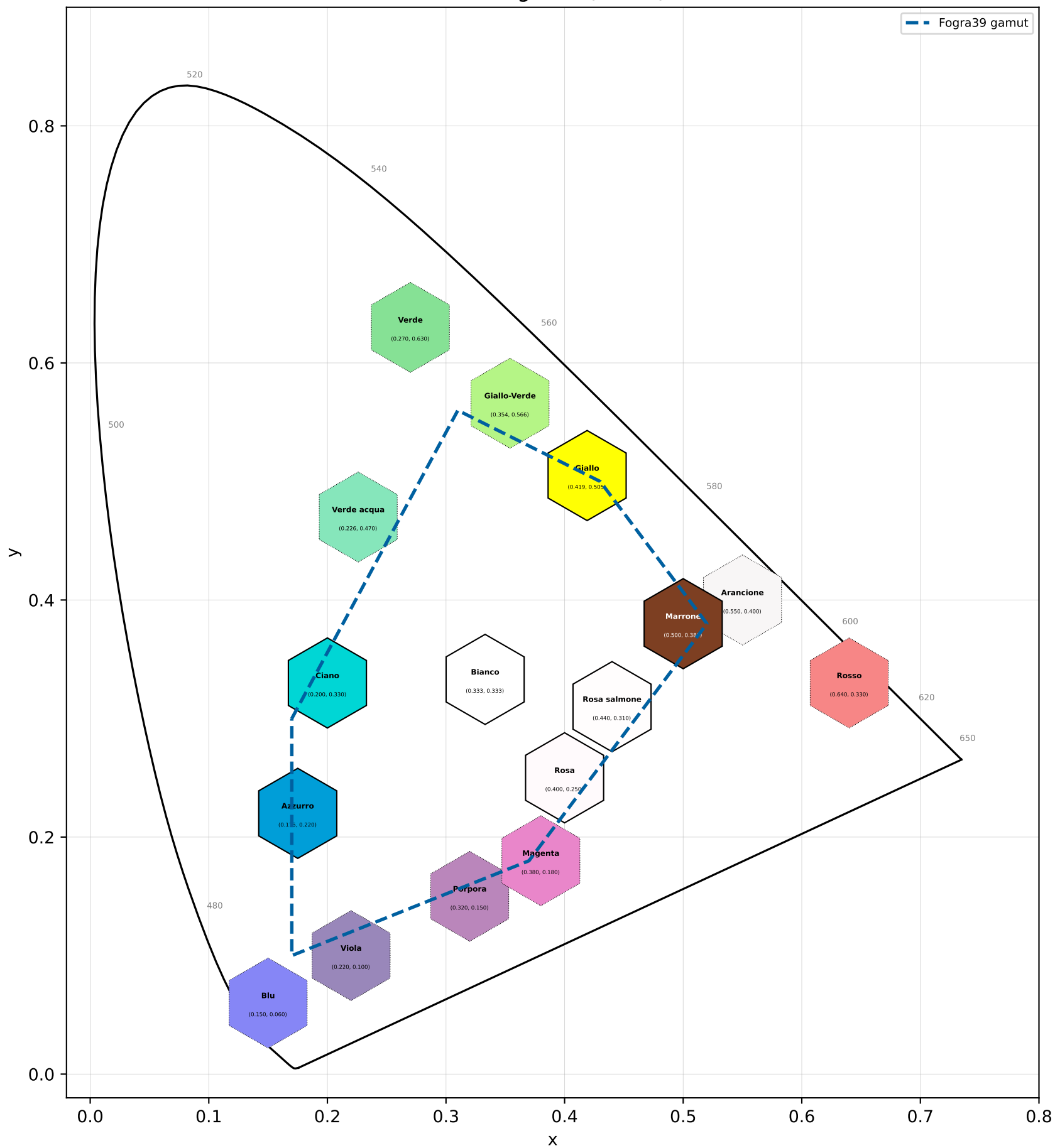
CIE 1931 — Fogra39 (CMYK) Gamut
