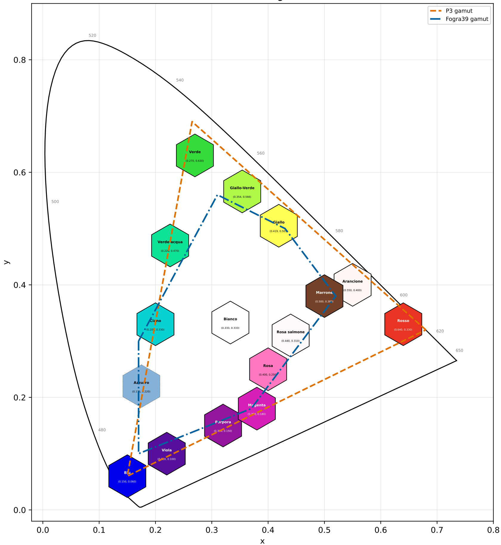
CIE 1931 — P3 + Fogra39 Gamuts
