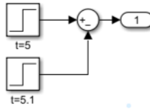
Figure 23: Disturbo a "spinta"
