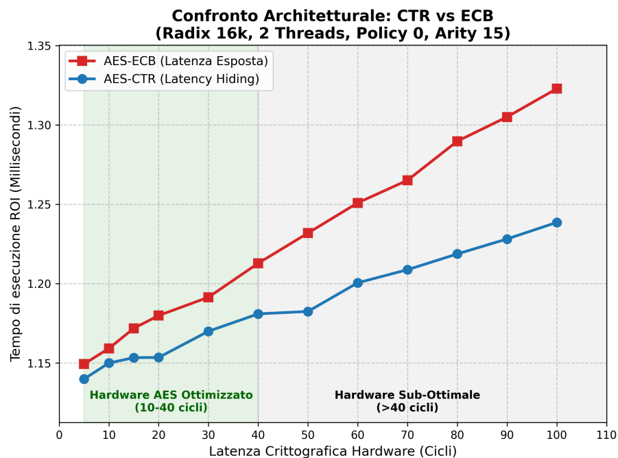
Figura 3.1: Latency Sweep
