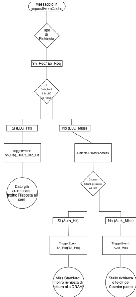
Figura 2.8: Flow Diagram RequestFromCache queue
