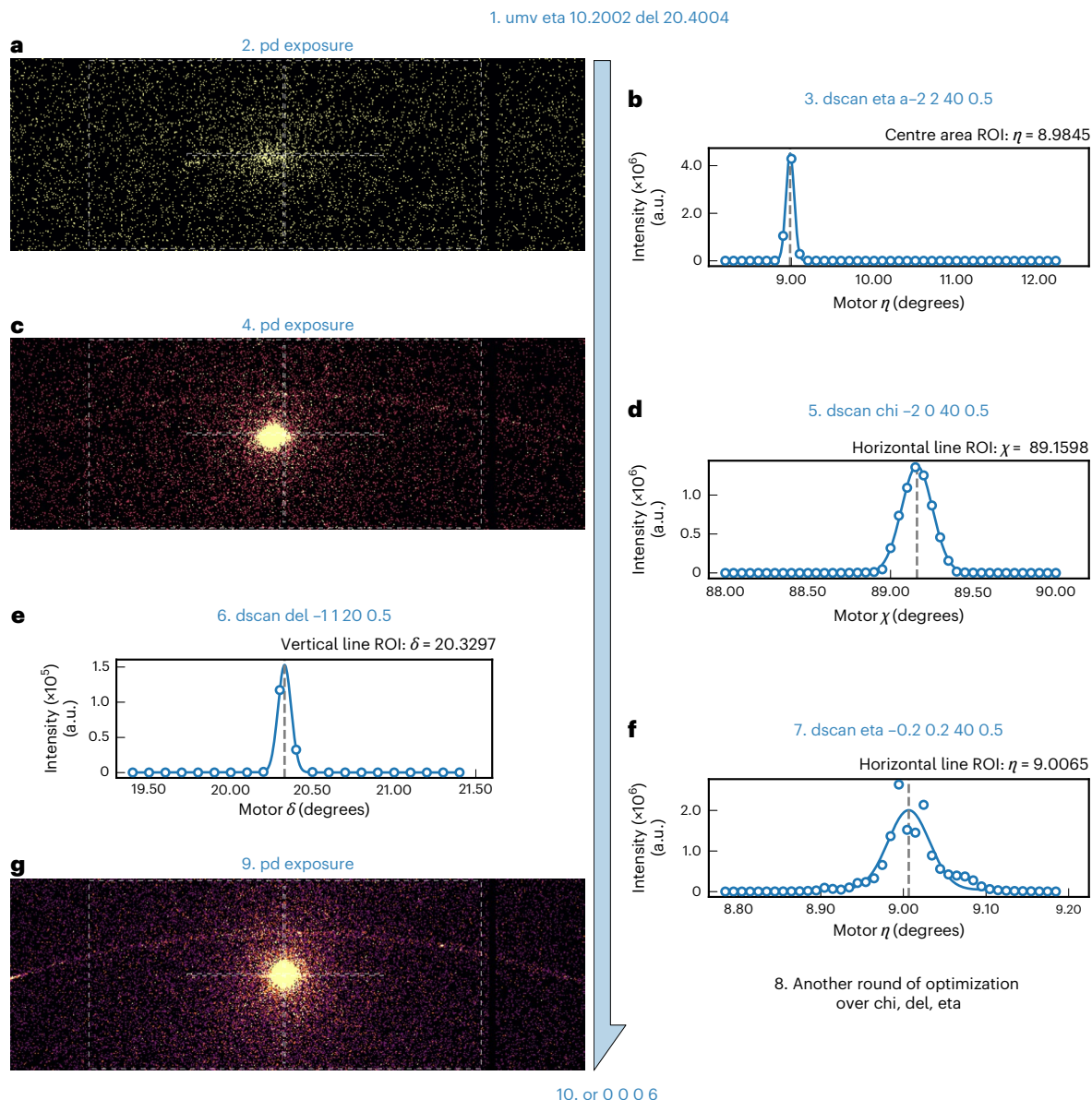
Fig. 3 | Key steps in finding and optimizing the first reference reflection, (0, 0, 6), for the \text{Co}_3\text{Sn}_2\text{S}_2 sample. a–g. Actions taken by the AI X-ray scientist include: capturing a detector image after moving motors \eta and \delta to the theoretical values for the (0, 0, 6) reflection (a); performing an \eta scan to optimize peak intensity (b); capturing a second detector image to verify the presence of the reflection (c); conducting a \chi scan to centre the peak horizontally (d), followed by a \delta scan to centre the peak vertically (e), and a final \eta scan for intensity optimization (f); and capturing the final detector image to confirm the optimized reflection before
