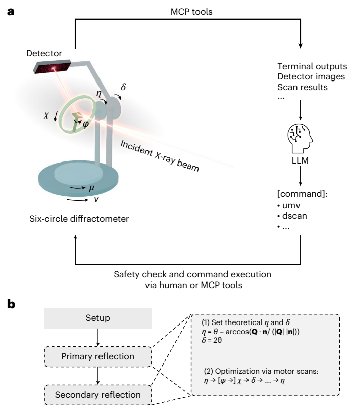
Fig. 1 | Schematic illustration of the AI X-ray scientist operating an X-ray scattering facility equipped with a six-circle (‘4S + 2D’) diffractometer.
