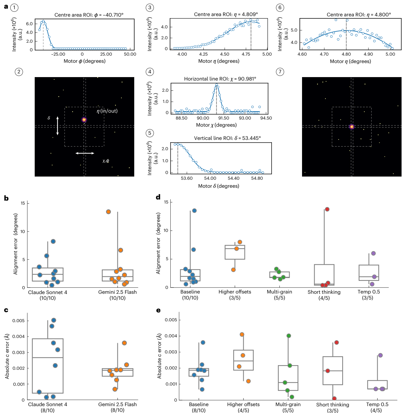
Fig. 2 | Autonomous sample orientation by the AIX-ray scientist in virtual experiments. a , Representative motor scans and detector image acquisitions performed by the AIX-ray scientist during a virtual single-crystal alignment procedure. Circular markers represent raw scan data, solid curves represent fitted peak profiles and vertical dashed lines indicate fitted peak positions. Detector images illustrate the corresponding diffraction patterns and regions of interest. Numbers 1–7 indicate the sequence of key actions during the procedure. b , Alignment error (in degrees) for sample orientation estimation across two agentic AI models. c , Absolute error in the estimated lattice constant c across the same two agentic AI models. d , Alignment error across different experimental conditions for the Gemini 2.5 Flash-based AIX-ray scientist, including baseline
