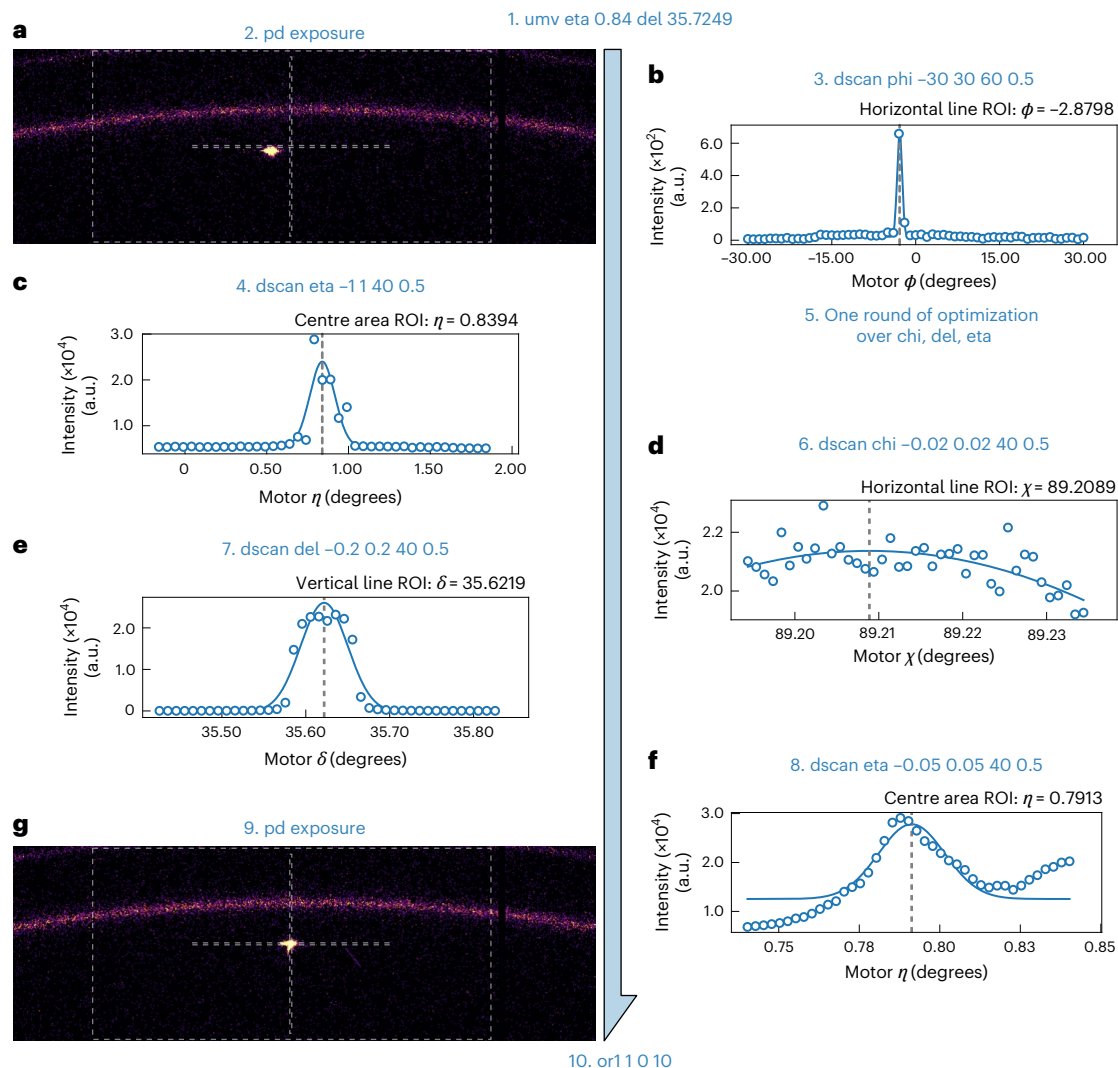
Fig. 4 | Key steps in finding and optimizing the second reference reflection, (1, 0, 10), from the \text{Co}_3\text{Sn}_2\text{S}_2 sample. This case highlights a challenging scenario where the AI X-ray scientist had no prior knowledge of the in-plane ( H - K ) orientation, which is a rare setup even in human-led experiments. Meanwhile, despite the presence of strong diffraction rings captured by the detector, the AI remained focused and successfully localized the Bragg peak. a–g , Actions taken include: capturing a detector image after moving motors \eta and \delta to the theoretical values for the (1, 0, 10) reflection ( a ); performing a wide \phi scan to determine the in-plane orientation ( b ); performing an \eta scan to optimize peak
