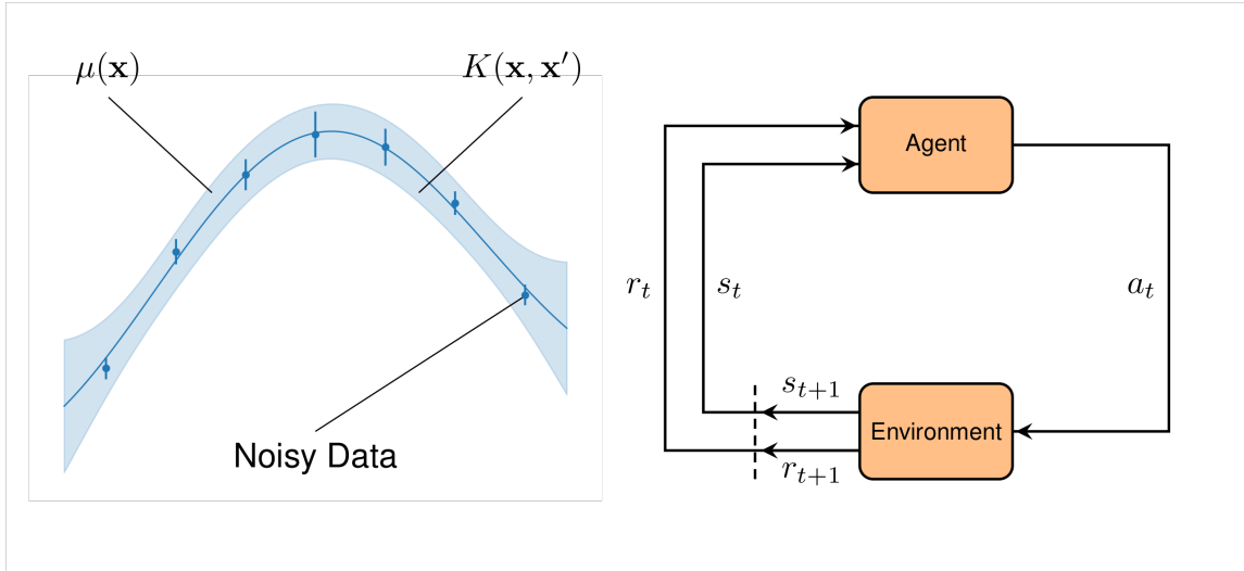
Figure 5: Bayesian Optimization and Reinforcement Learning. Bayesian Optimization approximates noisy data by fitting a Gaussian Process (left), which provides the mean function \mu(\mathbf{x}) and the kernel function K(\mathbf{x}, \mathbf{x}') for covariance. Reinforcement Learning (right) involves an agent interacting with the environment, where the agent, in state s_t , optimizes an action a_t to receive a reward r_t .
