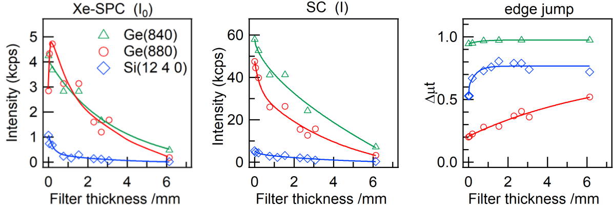
Fig. 4. Dependence of detected X-ray intensities at 25.4 keV on Al-filter thickness recorded with two different detectors and a monochromator crystal, and the resulting difference in the observed edge jump at Ag K-edge. Sample: 20 \mu\text{m} Ag foil.
