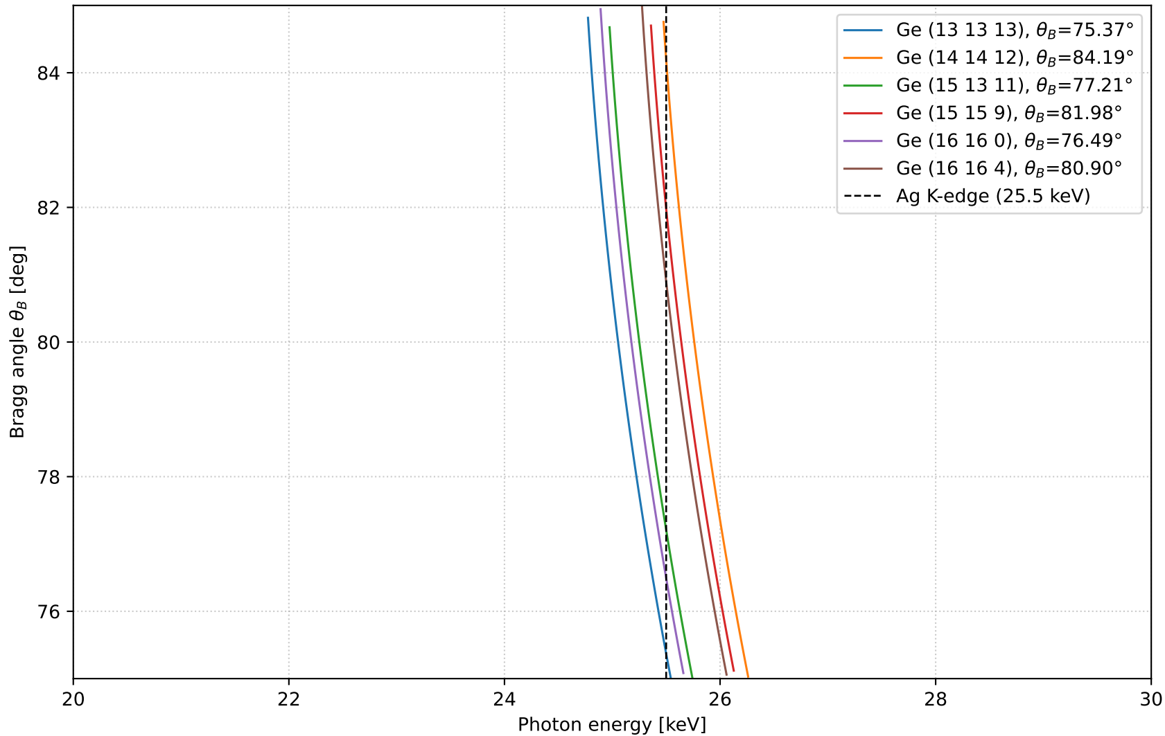
Ge reflections for Ag K-edge XANES (25.5 keV; 6 families)
